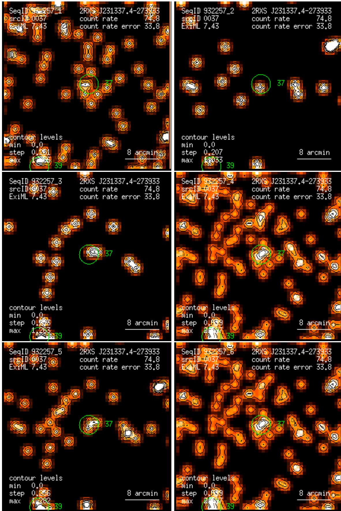
Figure 37: RASS 932257: detection 0037: band rate images, Gaussian filter: (1) PSPC channels 11 – 41, (2) 52 – 90, (3) 91 – 201, (4) 11 – 235, (5) 52 – 201, (6) 11 – 201. Broad band rates in counts/ks. Band rate contour levels in counts/ks/arcmin 2 .
