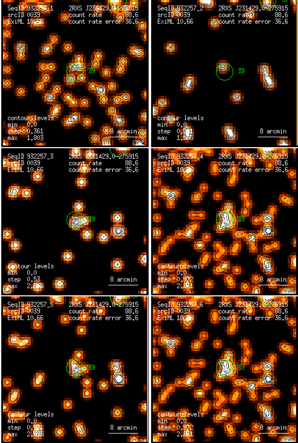
Figure 39: RASS 932257: detection 0039: band rate images, Gaussian filter: (1) PSPC channels 11 – 41, (2) 52 – 90, (3) 91 – 201, (4) 11 – 235, (5) 52 – 201, (6) 11 – 201. Broad band rates in counts/ks. Band rate contour levels in counts/ks/arcmin 2 .
