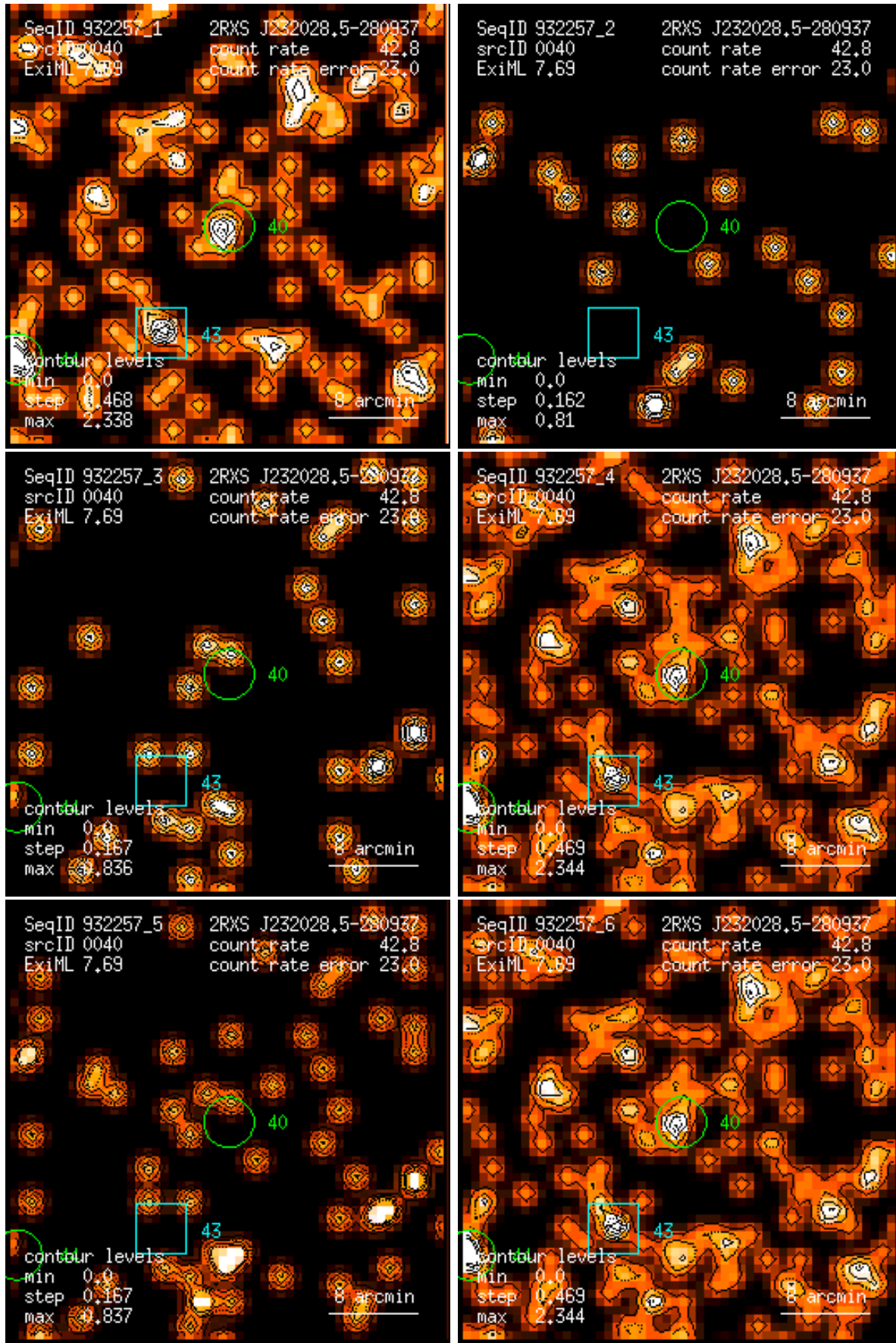
Figure 40: RASS 932257: detection 0040: band rate images, Gaussian filter: (1) PSPC channels 11 – 41, (2) 52 – 90, (3) 91 – 201, (4) 11 – 235, (5) 52 – 201, (6) 11 – 201. Broad band rates in counts/ks. Band rate contour levels in counts/ks/arcmin 2 .
