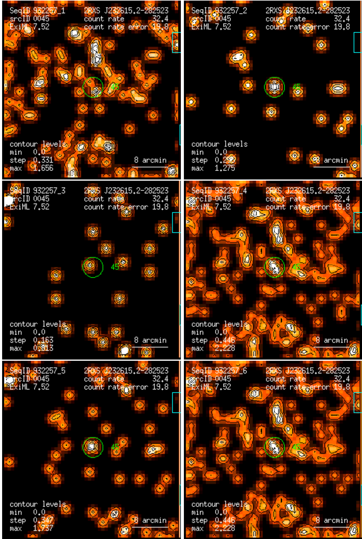
Figure 45: RASS 932257: detection 0045: band rate images, Gaussian filter: (1) PSPC channels 11 – 41, (2) 52 – 90, (3) 91 – 201, (4) 11 – 235, (5) 52 – 201, (6) 11 – 201. Broad band rates in counts/ks. Band rate contour levels in counts/ks/arcmin 2 .
