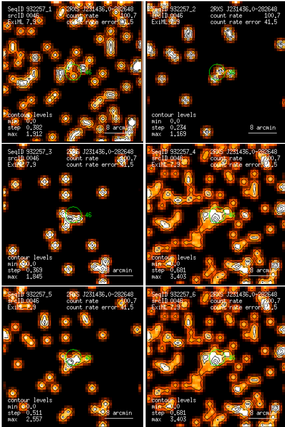
Figure 46: RASS 932257: detection 0046: band rate images, Gaussian filter: (1) PSPC channels 11 – 41, (2) 52 – 90, (3) 91 – 201, (4) 11 – 235, (5) 52 – 201, (6) 11 – 201. Broad band rates in counts/ks. Band rate contour levels in counts/ks/arcmin 2 .
