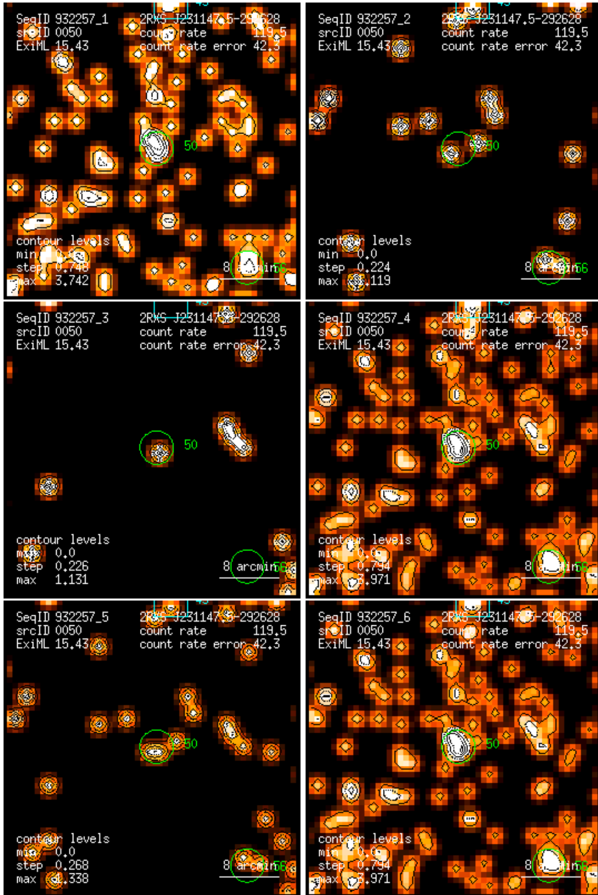
Figure 50: RASS 932257: detection 0050: band rate images, Gaussian filter: (1) PSPC channels 11 – 41, (2) 52 – 90, (3) 91 – 201, (4) 11 – 235, (5) 52 – 201, (6) 11 – 201. Broad band rates in counts/ks. Band rate contour levels in counts/ks/arcmin 2 .
