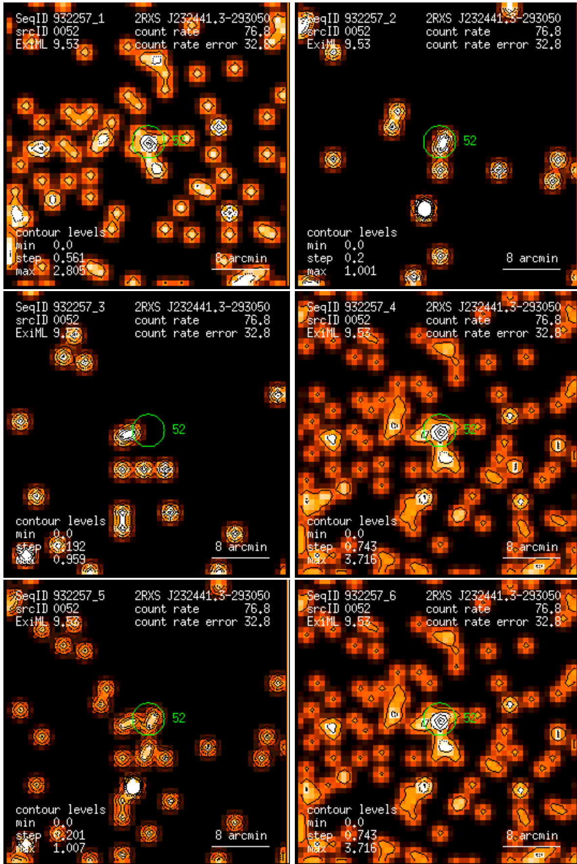
Figure 52: RASS 932257: detection 0052: band rate images, Gaussian filter: (1) PSPC channels 11 – 41, (2) 52 – 90, (3) 91 – 201, (4) 11 – 235, (5) 52 – 201, (6) 11 – 201. Broad band rates in counts/ks. Band rate contour levels in counts/ks/arcmin 2 .
