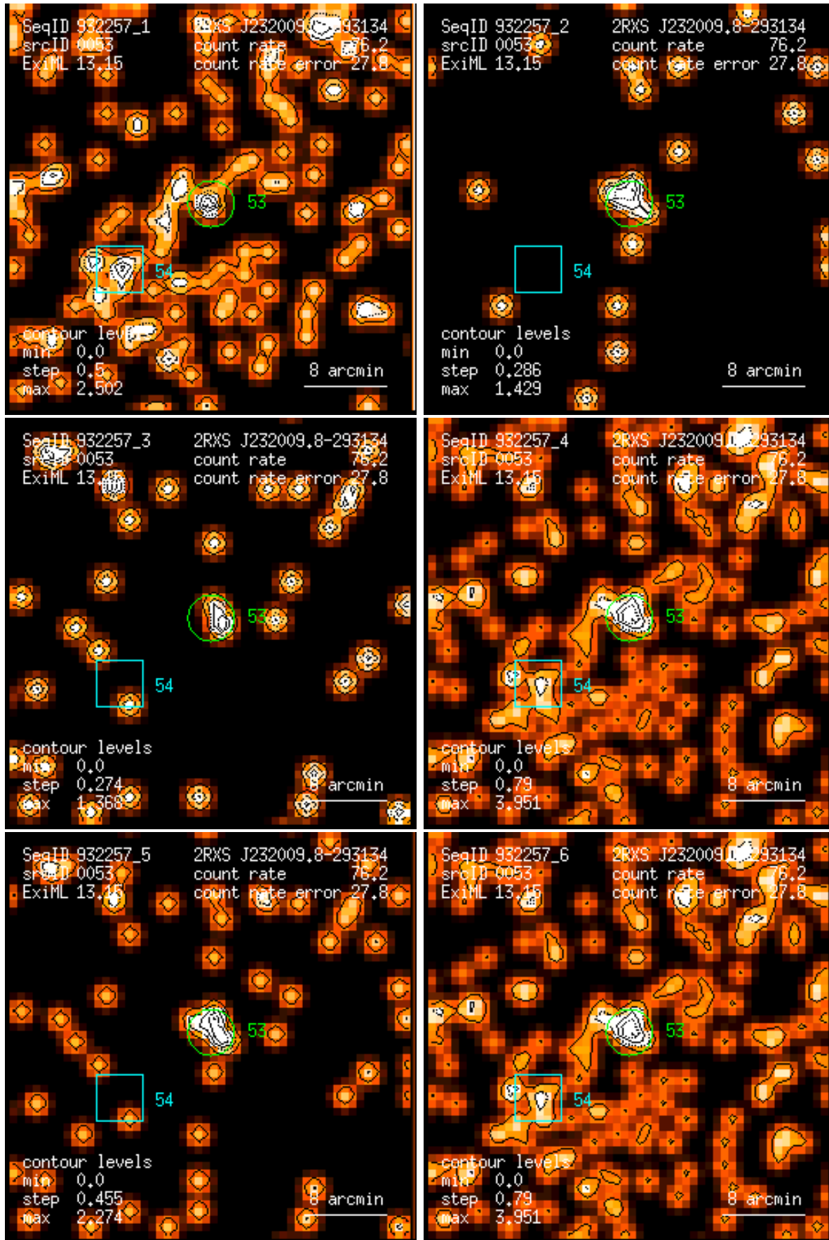
Figure 53: RASS 932257: detection 0053: band rate images, Gaussian filter: (1) PSPC channels 11 – 41, (2) 52 – 90, (3) 91 – 201, (4) 11 – 235, (5) 52 – 201, (6) 11 – 201. Broad band rates in counts/ks. Band rate contour levels in counts/ks/arcmin 2 .
