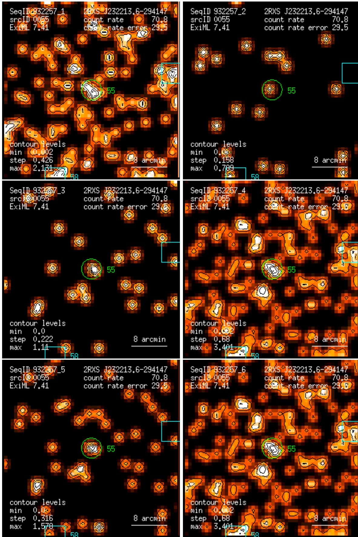
Figure 55: RASS 932257: detection 0055: band rate images, Gaussian filter: (1) PSPC channels 11 – 41, (2) 52 – 90, (3) 91 – 201, (4) 11 – 235, (5) 52 – 201, (6) 11 – 201. Broad band rates in counts/ks. Band rate contour levels in counts/ks/arcmin 2 .
