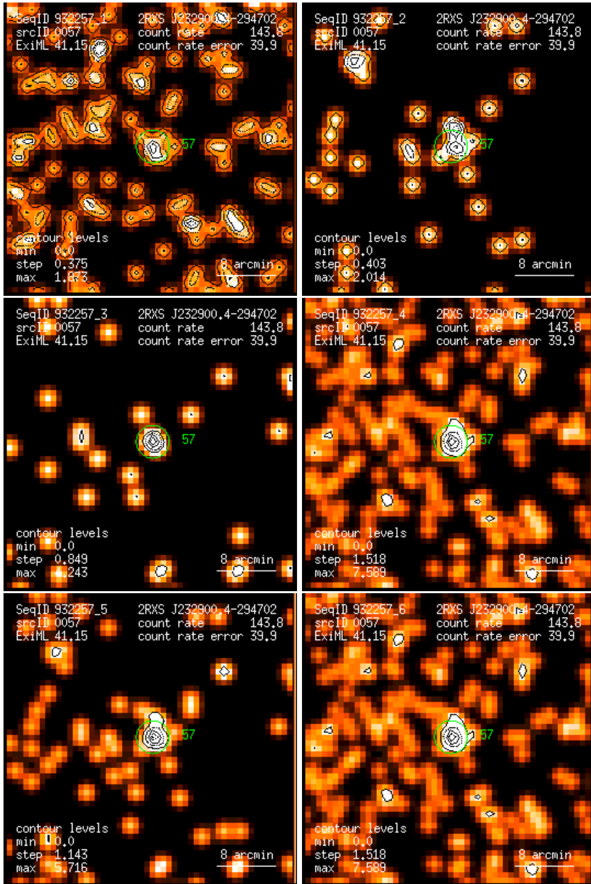
Figure 57: RASS 932257: detection 0057: band rate images, Gaussian filter: (1) PSPC channels 11 – 41, (2) 52 – 90, (3) 91 – 201, (4) 11 – 235, (5) 52 – 201, (6) 11 – 201. Broad band rates in counts/ks. Band rate contour levels in counts/ks/arcmin 2 .
