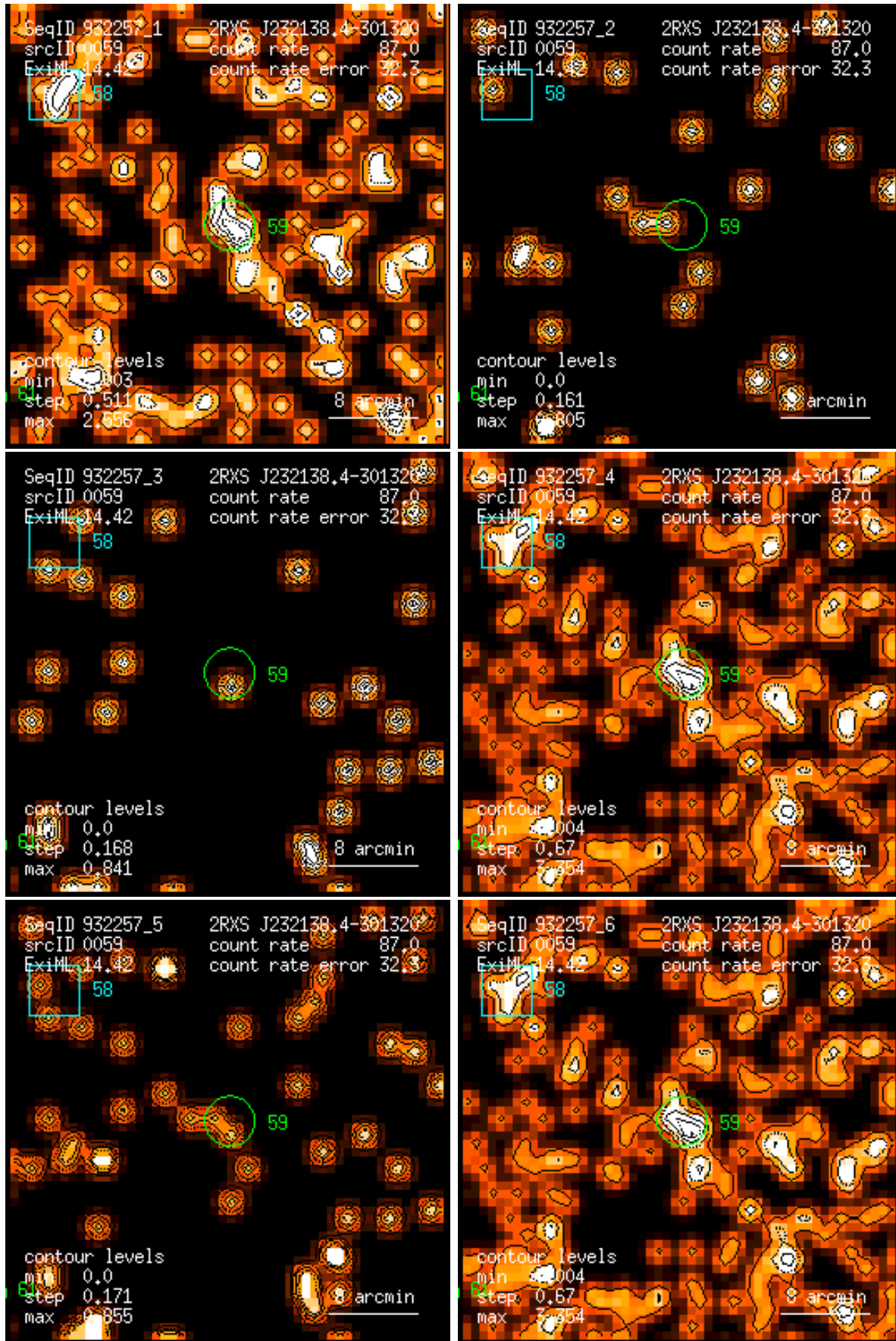
Figure 59: RASS 932257: detection 0059: band rate images, Gaussian filter: (1) PSPC channels 11 – 41, (2) 52 – 90, (3) 91 – 201, (4) 11 – 235, (5) 52 – 201, (6) 11 – 201. Broad band rates in counts/ks. Band rate contour levels in counts/ks/arcmin 2 .
