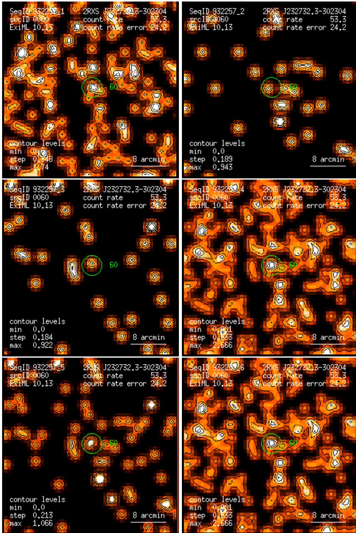
Figure 60: RASS 932257: detection 0060: band rate images, Gaussian filter: (1) PSPC channels 11 – 41, (2) 52 – 90, (3) 91 – 201, (4) 11 – 235, (5) 52 – 201, (6) 11 – 201. Broad band rates in counts/ks. Band rate contour levels in counts/ks/arcmin 2 .
