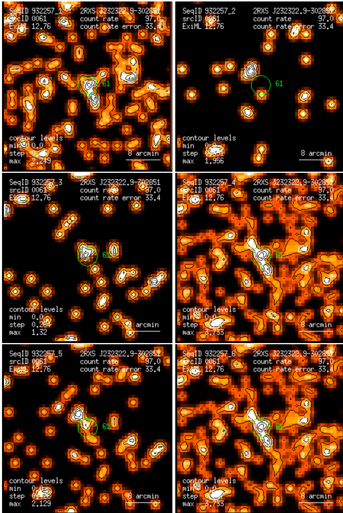
Figure 61: RASS 932257: detection 0061: band rate images, Gaussian filter: (1) PSPC channels 11 – 41, (2) 52 – 90, (3) 91 – 201, (4) 11 – 235, (5) 52 – 201, (6) 11 – 201. Broad band rates in counts/ks. Band rate contour levels in counts/ks/arcmin 2 .
