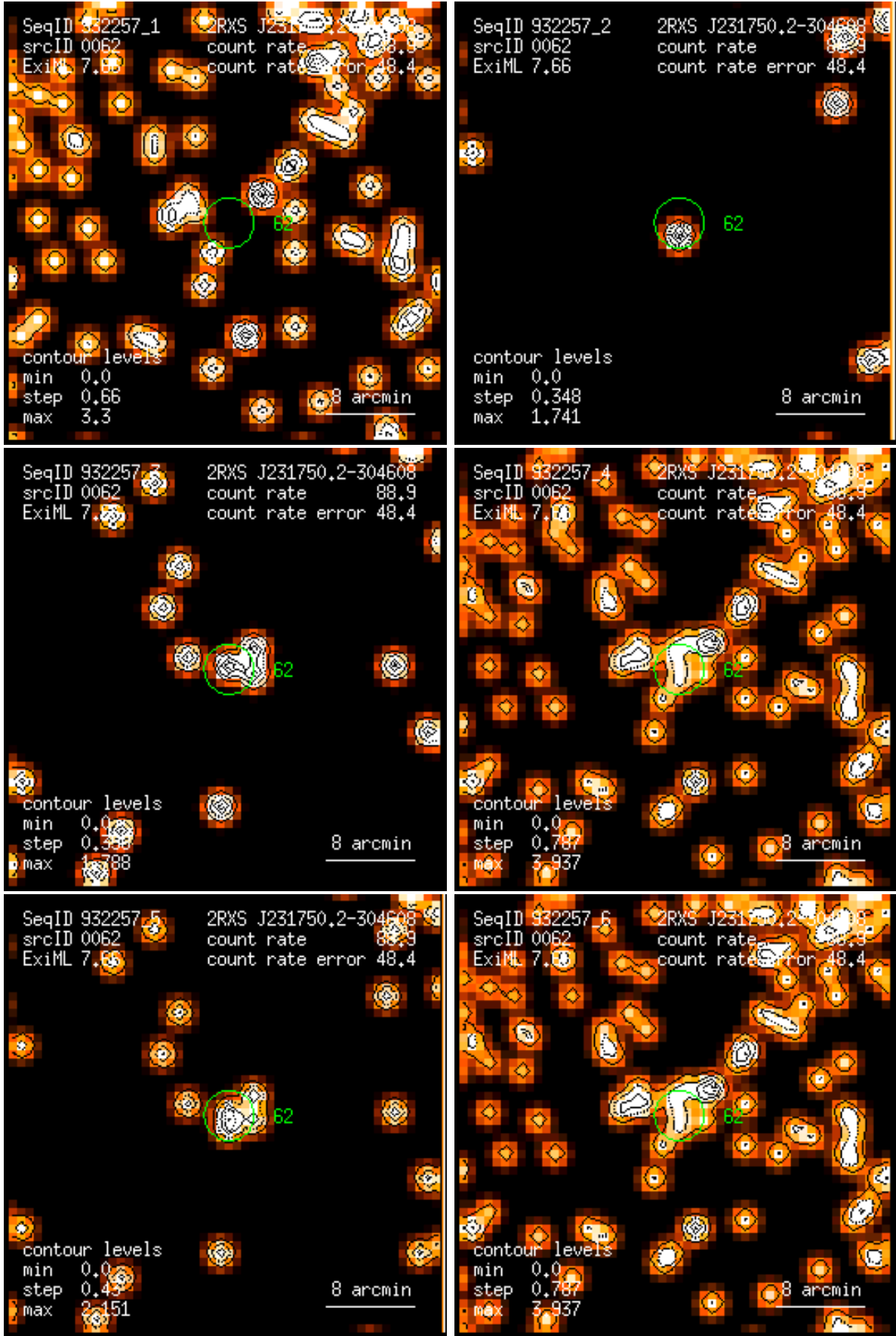
Figure 62: RASS 932257: detection 0062: band rate images, Gaussian filter: (1) PSPC channels 11 – 41, (2) 52 – 90, (3) 91 – 201, (4) 11 – 235, (5) 52 – 201, (6) 11 – 201. Broad band rates in counts/ks. Band rate contour levels in counts/ks/arcmin 2 .
