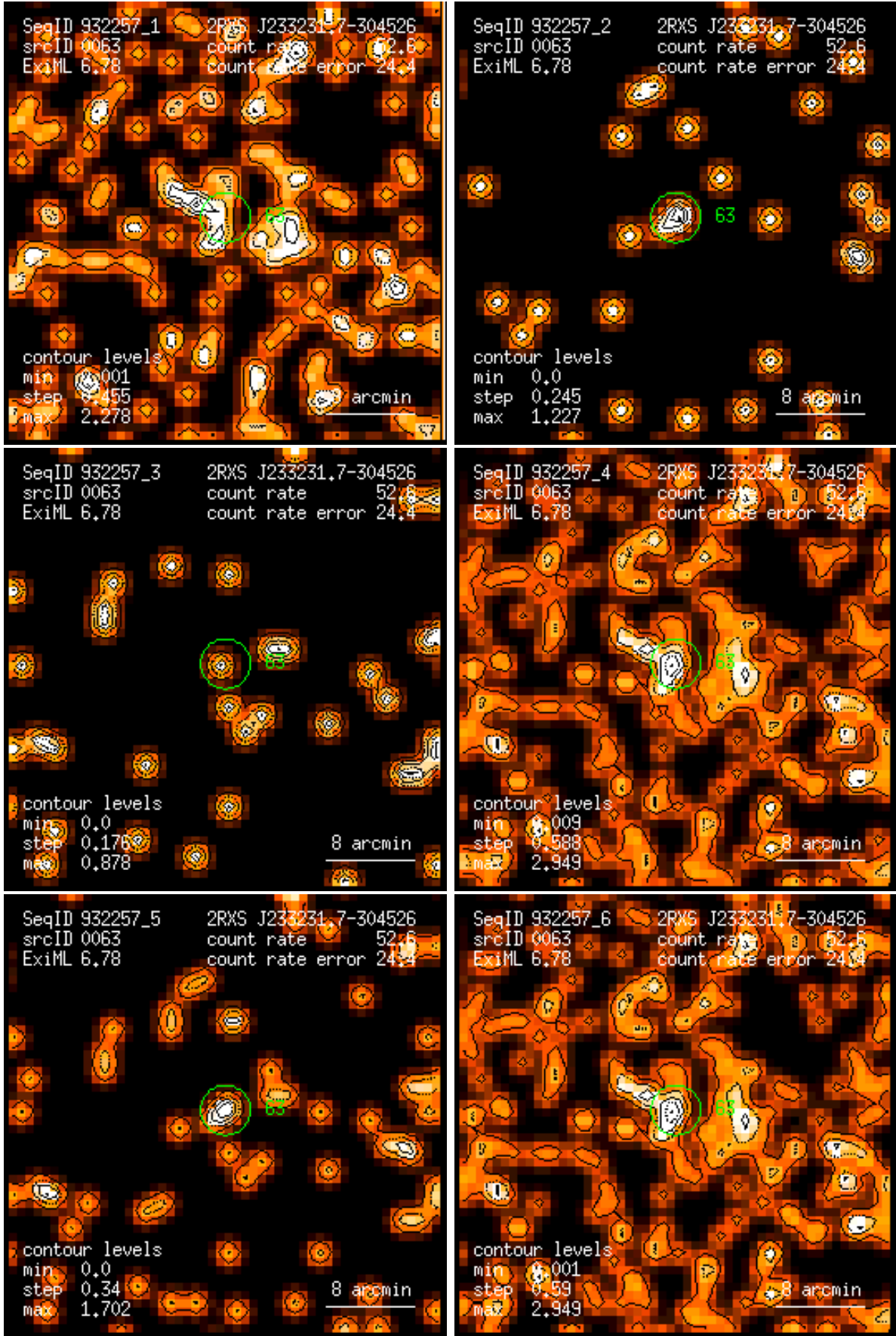
Figure 63: RASS 932257: detection 0063: band rate images, Gaussian filter: (1) PSPC channels 11 – 41, (2) 52 – 90, (3) 91 – 201, (4) 11 – 235, (5) 52 – 201, (6) 11 – 201. Broad band rates in counts/ks. Band rate contour levels in counts/ks/arcmin 2 .
