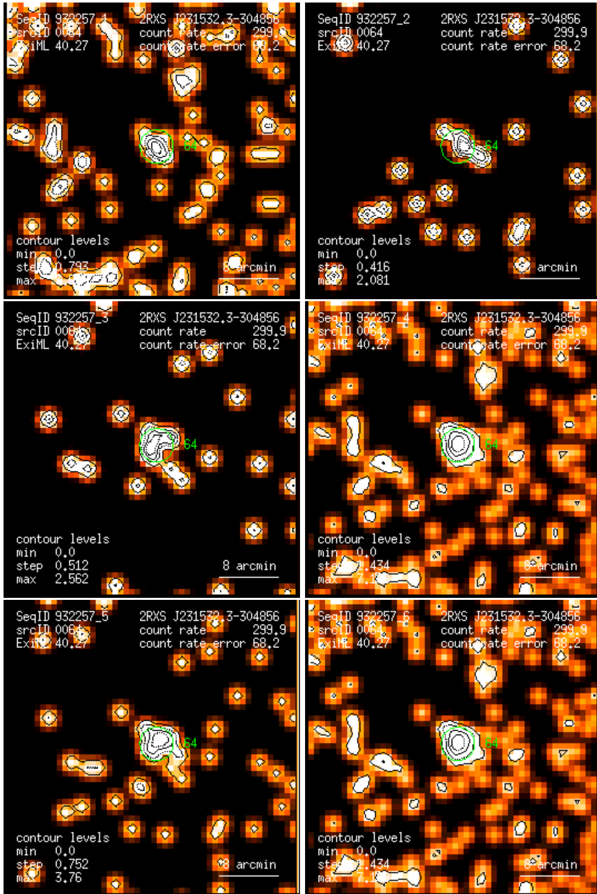
Figure 64: RASS 932257: detection 0064: band rate images, Gaussian filter: (1) PSPC channels 11 – 41, (2) 52 – 90, (3) 91 – 201, (4) 11 – 235, (5) 52 – 201, (6) 11 – 201. Broad band rates in counts/ks. Band rate contour levels in counts/ks/arcmin 2 .
