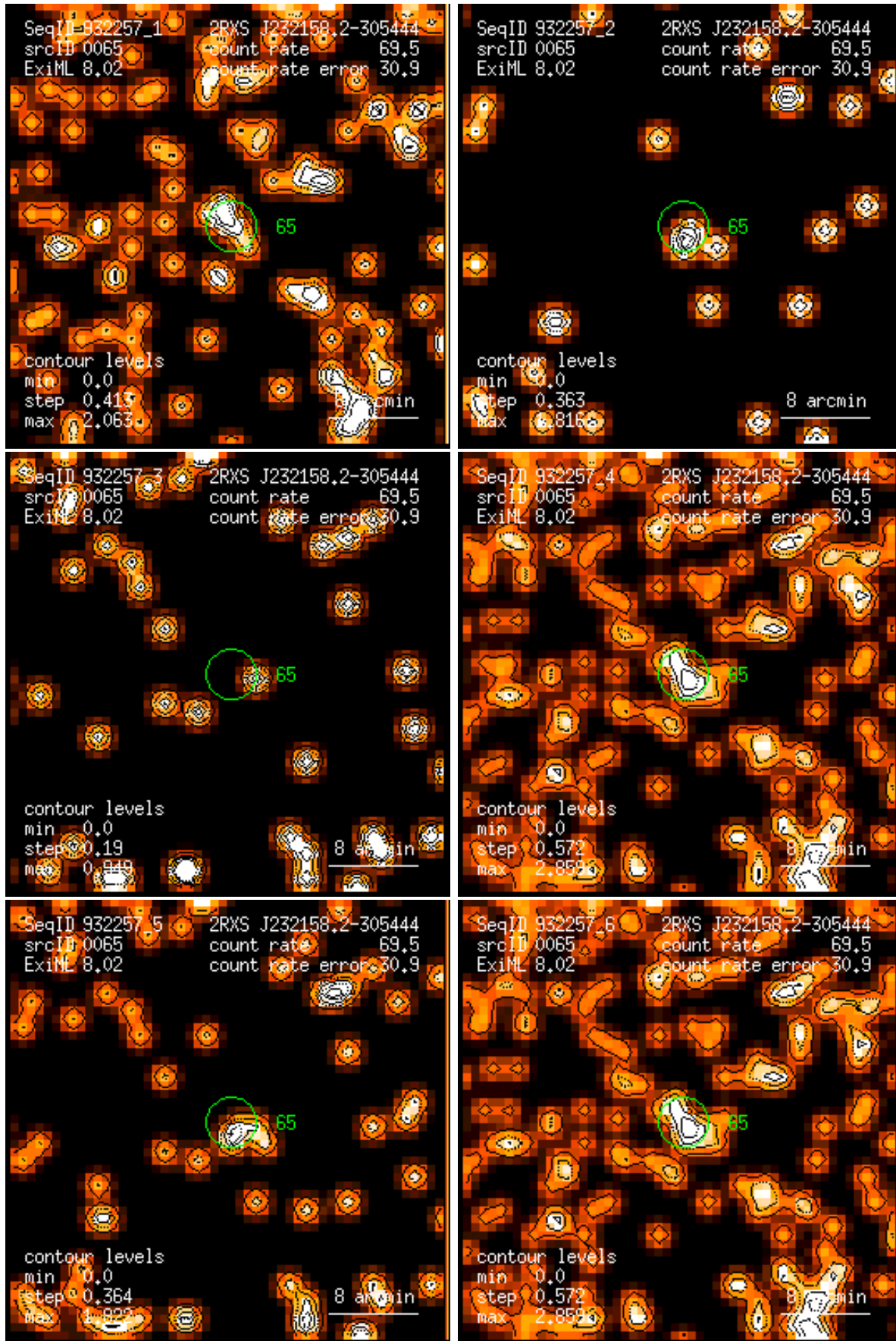
Figure 65: RASS 932257: detection 0065: band rate images, Gaussian filter: (1) PSPC channels 11 – 41, (2) 52 – 90, (3) 91 – 201, (4) 11 – 235, (5) 52 – 201, (6) 11 – 201. Broad band rates in counts/ks. Band rate contour levels in counts/ks/arcmin 2 .
