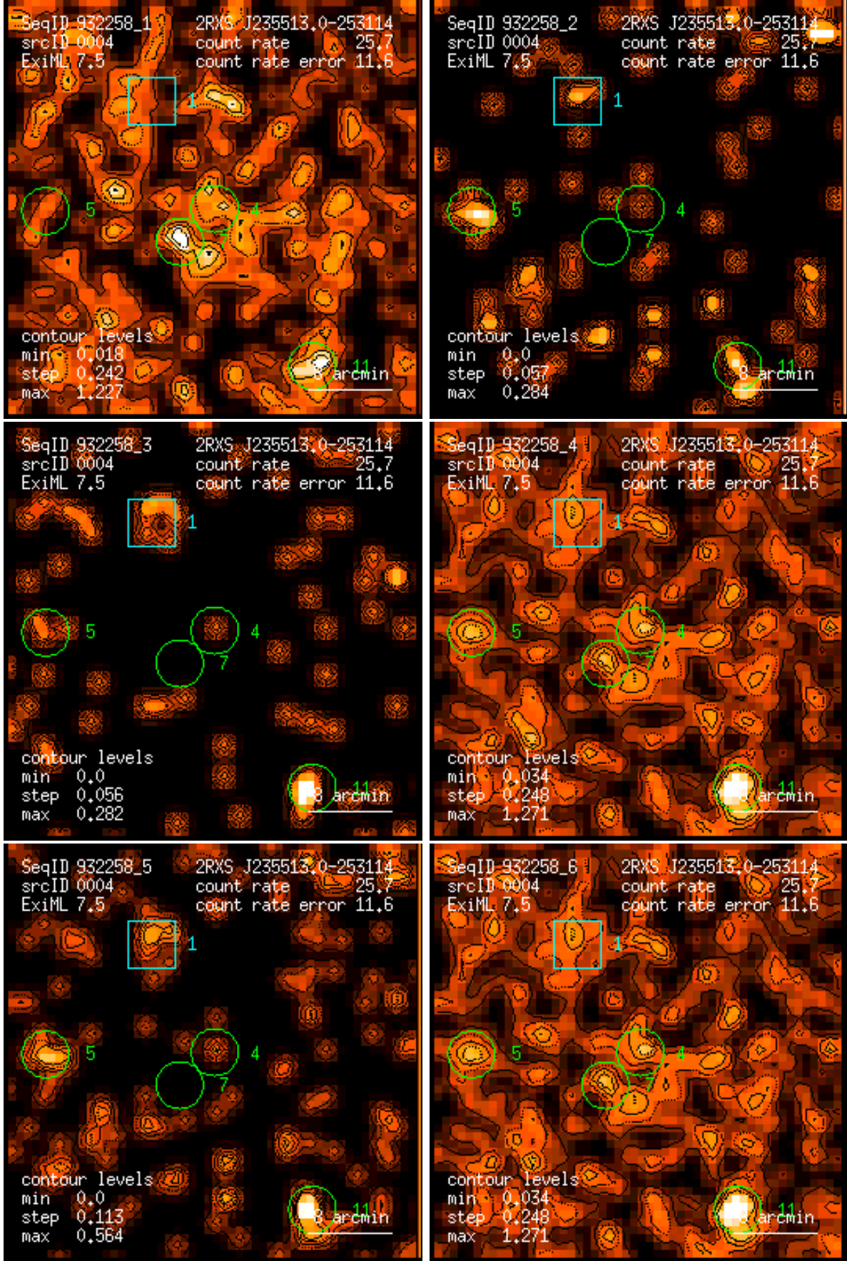
Figure 4: RASS 932258: detection 0004: band rate images, Gaussian filter: (1) PSPC channels 11 – 41, (2) 52 – 90, (3) 91 – 201, (4) 11 – 235, (5) 52 – 201, (6) 11 – 201. Broad band rates in counts/ks. Band rate contour levels in counts/ks/arcmin 2 .
