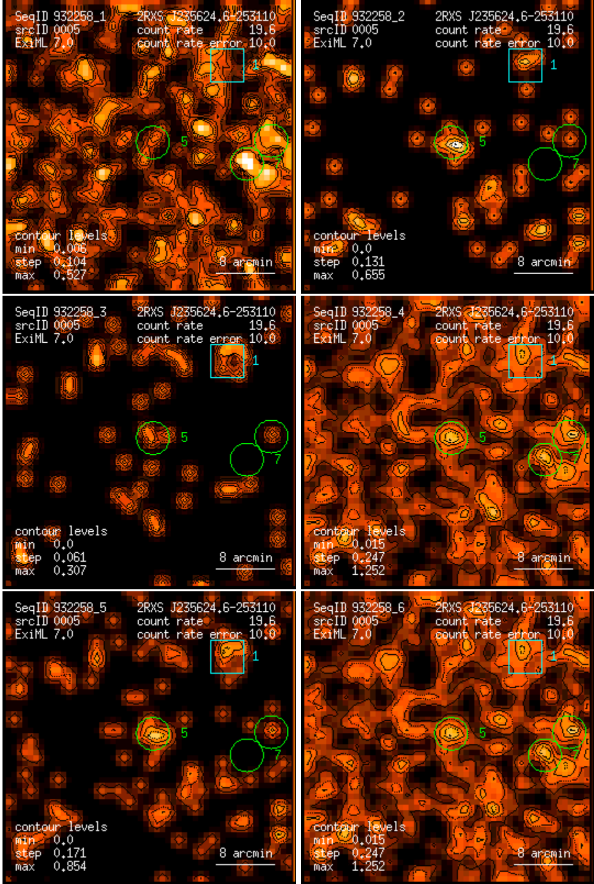
Figure 5: RASS 932258: detection 0005: band rate images, Gaussian filter: (1) PSPC channels 11 – 41, (2) 52 – 90, (3) 91 – 201, (4) 11 – 235, (5) 52 – 201, (6) 11 – 201. Broad band rates in counts/ks. Band rate contour levels in counts/ks/arcmin 2 .
