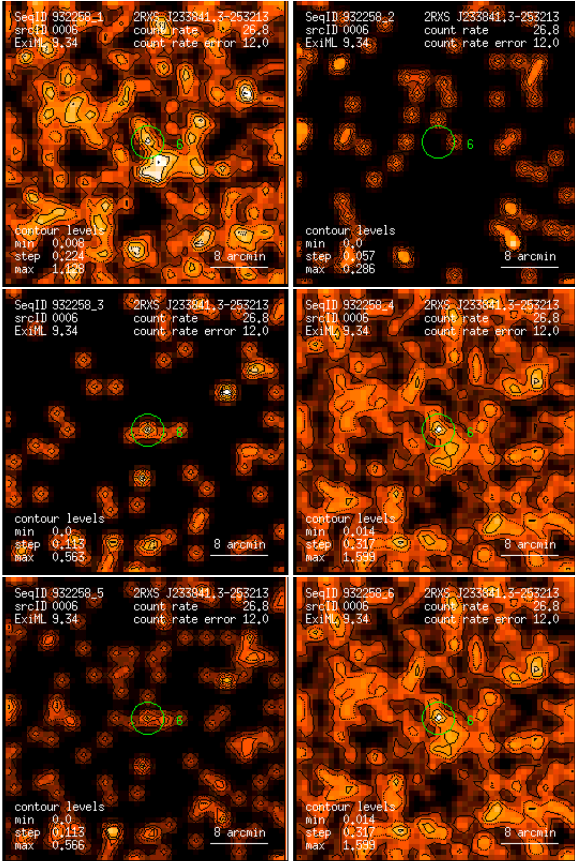
Figure 6: RASS 932258: detection 0006: band rate images, Gaussian filter: (1) PSPC channels 11 – 41, (2) 52 – 90, (3) 91 – 201, (4) 11 – 235, (5) 52 – 201, (6) 11 – 201. Broad band rates in counts/ks. Band rate contour levels in counts/ks/arcmin 2 .
