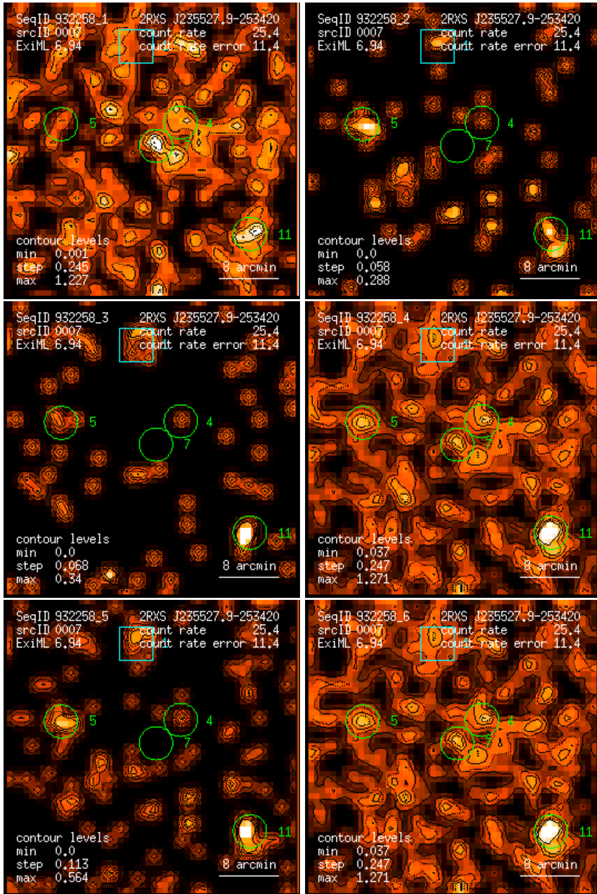
Figure 7: RASS 932258: detection 0007: band rate images, Gaussian filter: (1) PSPC channels 11 – 41, (2) 52 – 90, (3) 91 – 201, (4) 11 – 235, (5) 52 – 201, (6) 11 – 201. Broad band rates in counts/ks. Band rate contour levels in counts/ks/arcmin 2 .
