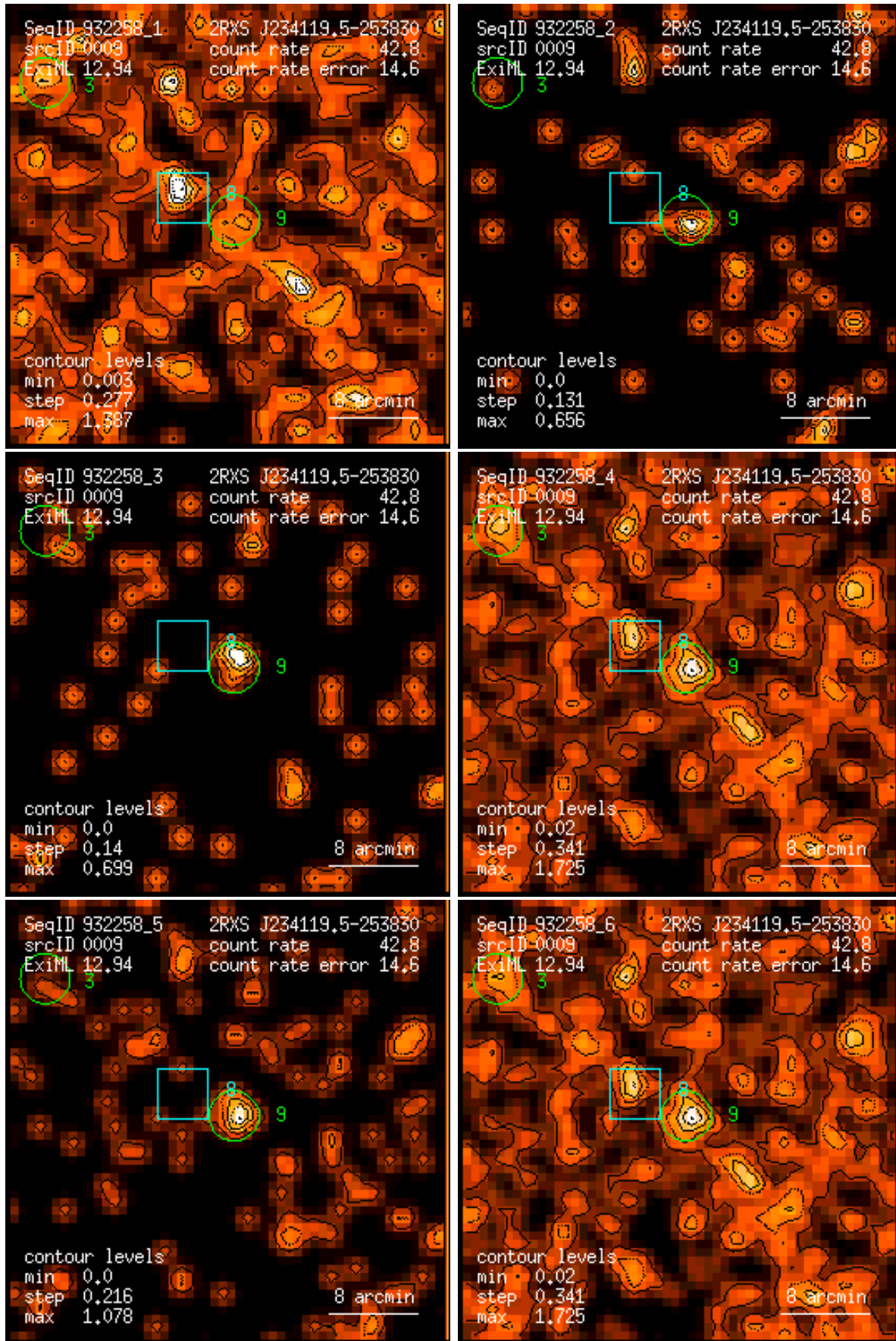
Figure 9: RASS 932258: detection 0009: band rate images, Gaussian filter: (1) PSPC channels 11 – 41, (2) 52 – 90, (3) 91 – 201, (4) 11 – 235, (5) 52 – 201, (6) 11 – 201. Broad band rates in counts/ks. Band rate contour levels in counts/ks/arcmin 2 .
