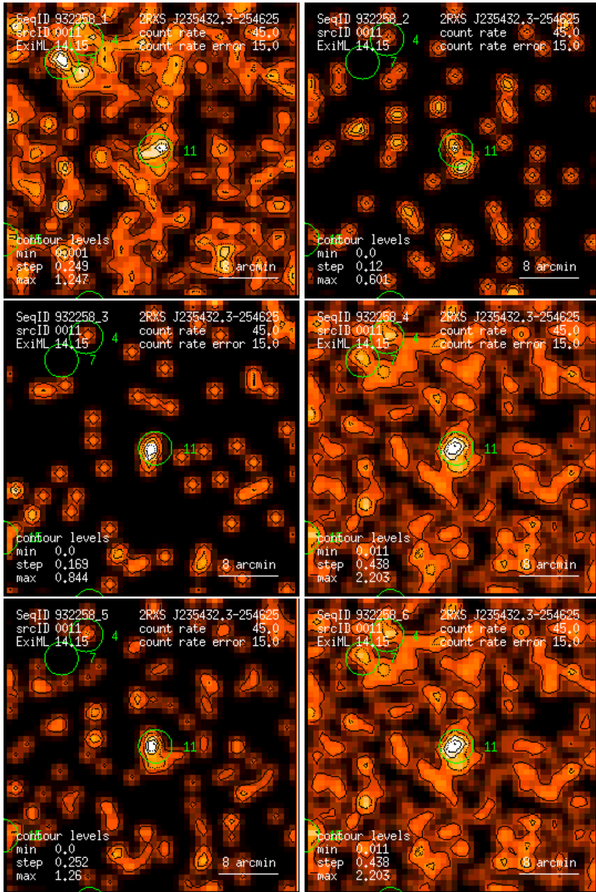
Figure 11: RASS 932258: detection 0011: band rate images, Gaussian filter: (1) PSPC channels 11 – 41, (2) 52 – 90, (3) 91 – 201, (4) 11 – 235, (5) 52 – 201, (6) 11 – 201. Broad band rates in counts/ks. Band rate contour levels in counts/ks/arcmin 2 .
