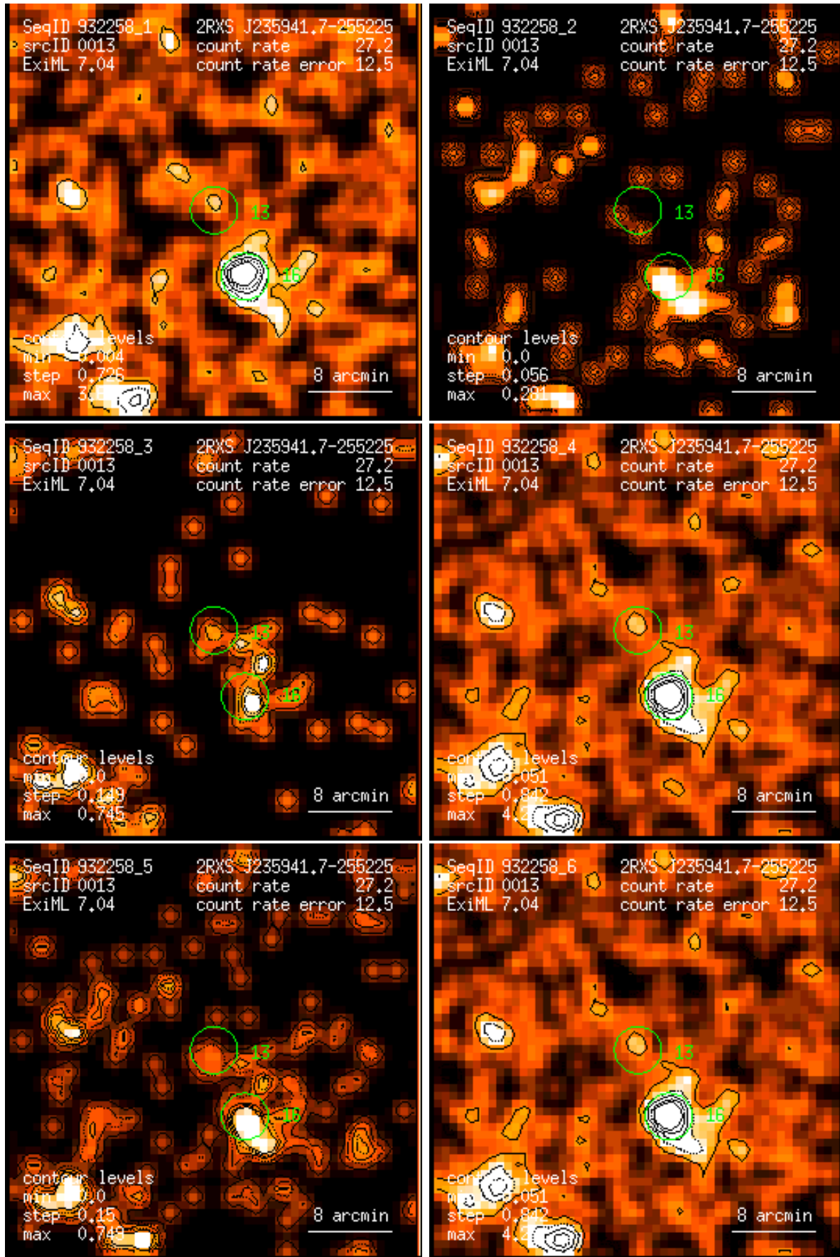
Figure 13: RASS 932258: detection 0013: band rate images, Gaussian filter: (1) PSPC channels 11 – 41, (2) 52 – 90, (3) 91 – 201, (4) 11 – 235, (5) 52 – 201, (6) 11 – 201. Broad band rates in counts/ks. Band rate contour levels in counts/ks/arcmin 2 .
