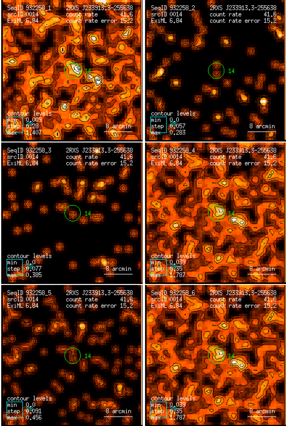
Figure 14: RASS 932258: detection 0014: band rate images, Gaussian filter: (1) PSPC channels 11 – 41, (2) 52 – 90, (3) 91 – 201, (4) 11 – 235, (5) 52 – 201, (6) 11 – 201. Broad band rates in counts/ks. Band rate contour levels in counts/ks/arcmin 2 .
