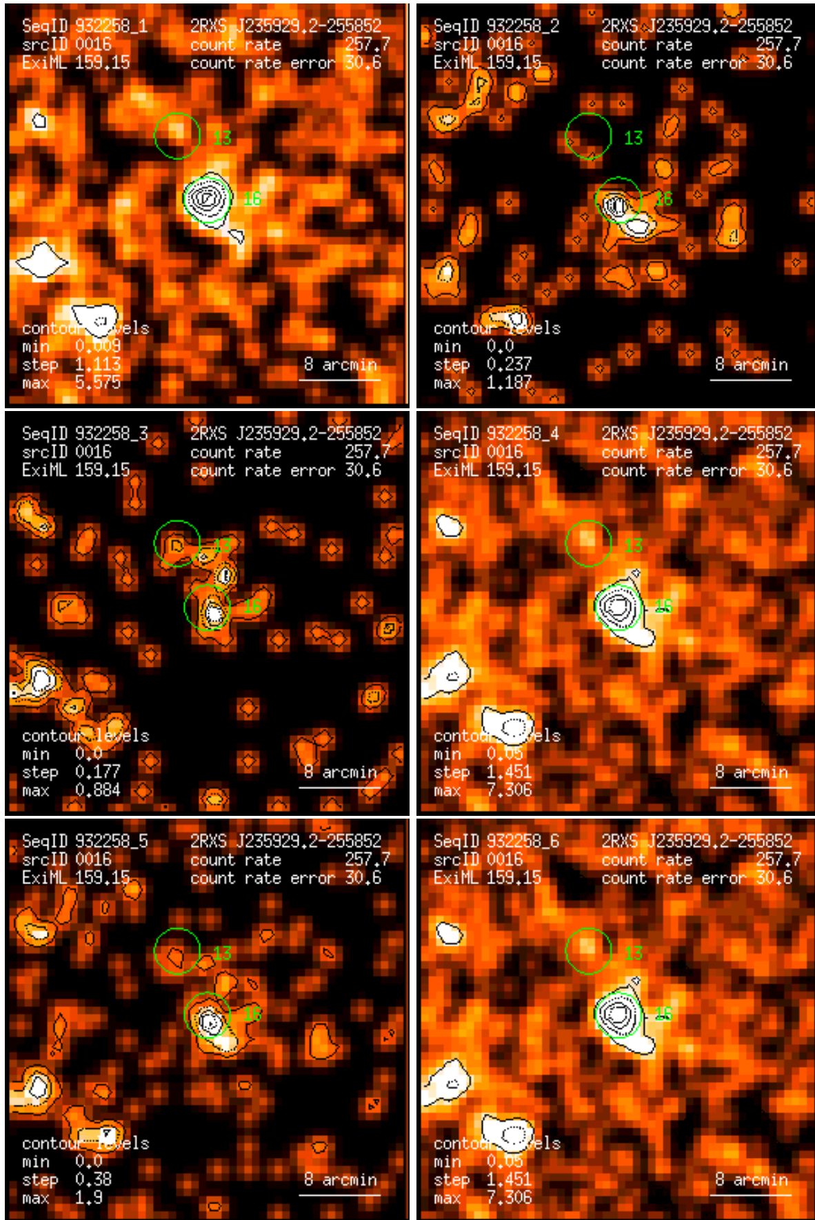
Figure 16: RASS 932258: detection 0016: band rate images, Gaussian filter: (1) PSPC channels 11 – 41, (2) 52 – 90, (3) 91 – 201, (4) 11 – 235, (5) 52 – 201, (6) 11 – 201. Broad band rates in counts/ks. Band rate contour levels in counts/ks/arcmin 2 .
