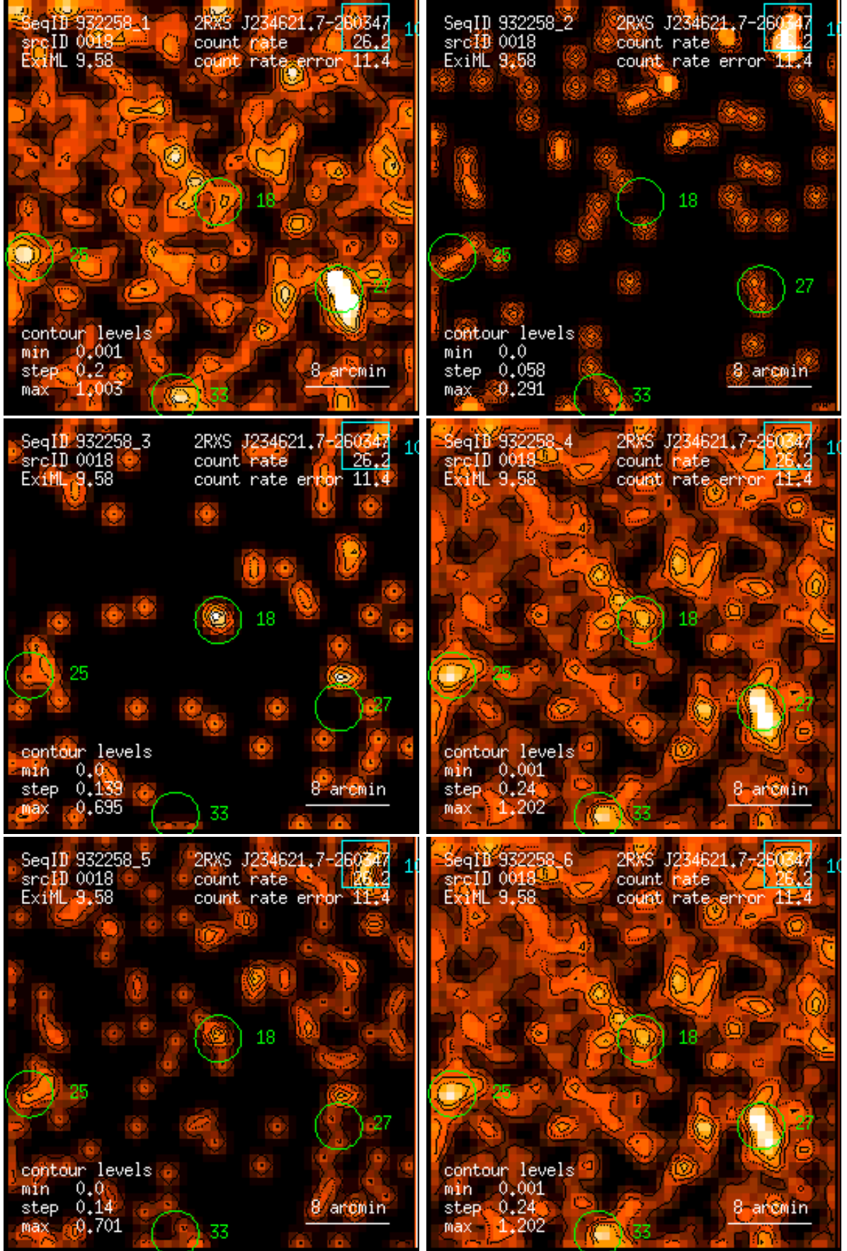
Figure 18: RASS 932258: detection 0018: band rate images, Gaussian filter: (1) PSPC channels 11 – 41, (2) 52 – 90, (3) 91 – 201, (4) 11 – 235, (5) 52 – 201, (6) 11 – 201. Broad band rates in counts/ks. Band rate contour levels in counts/ks/arcmin 2 .
