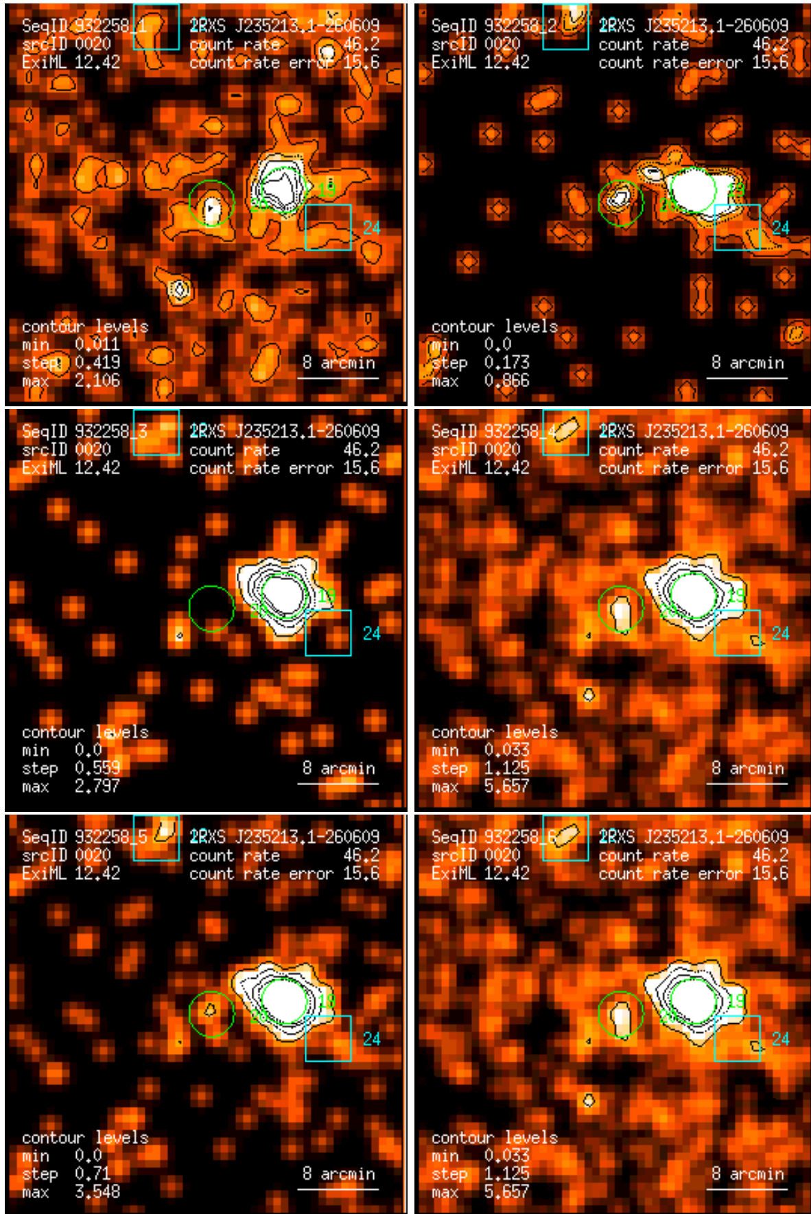
Figure 20: RASS 932258: detection 0020: band rate images, Gaussian filter: (1) PSPC channels 11 – 41, (2) 52 – 90, (3) 91 – 201, (4) 11 – 235, (5) 52 – 201, (6) 11 – 201. Broad band rates in counts/ks. Band rate contour levels in counts/ks/arcmin 2 .
