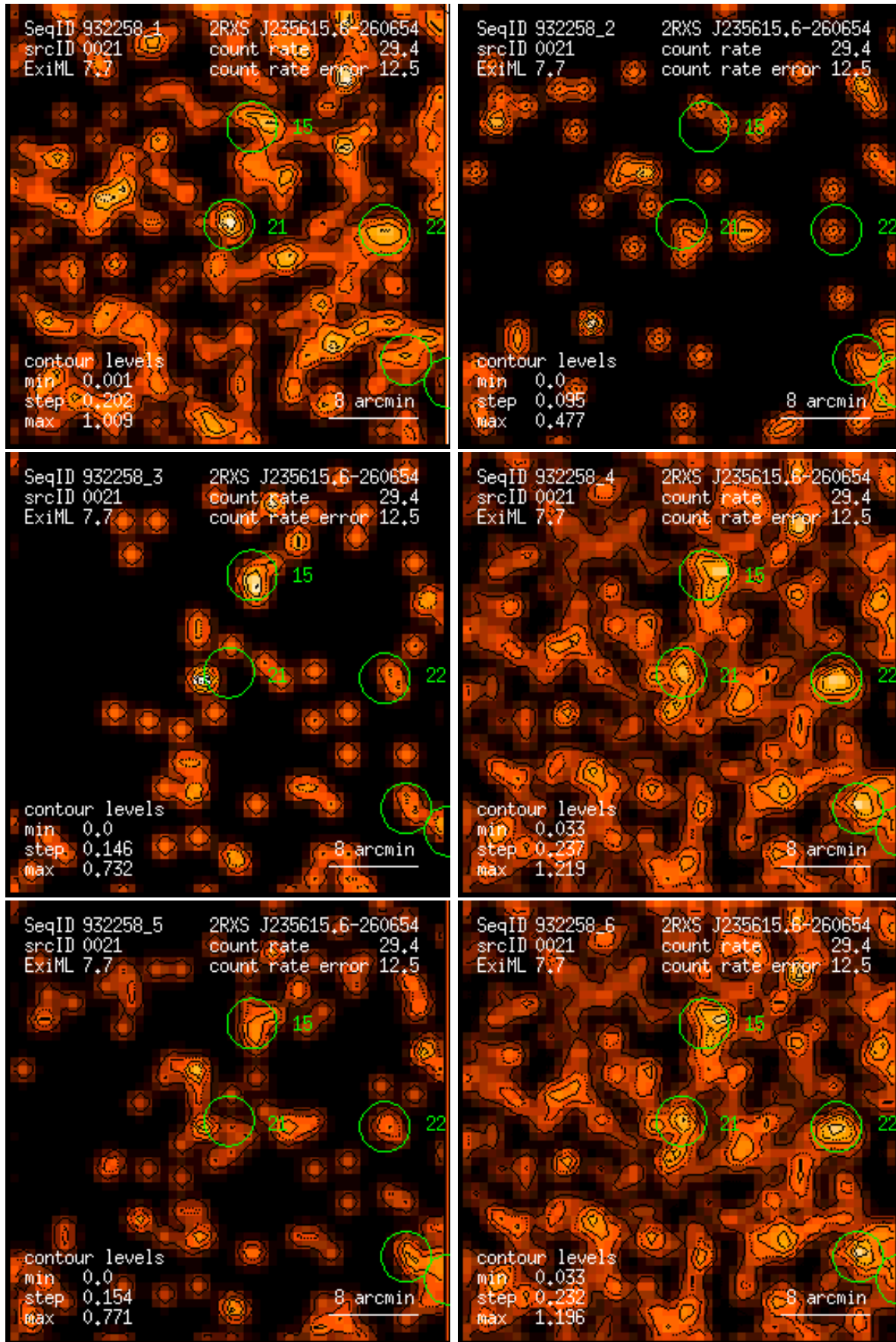
Figure 21: RASS 932258: detection 0021: band rate images, Gaussian filter: (1) PSPC channels 11 – 41, (2) 52 – 90, (3) 91 – 201, (4) 11 – 235, (5) 52 – 201, (6) 11 – 201. Broad band rates in counts/ks. Band rate contour levels in counts/ks/arcmin 2 .
