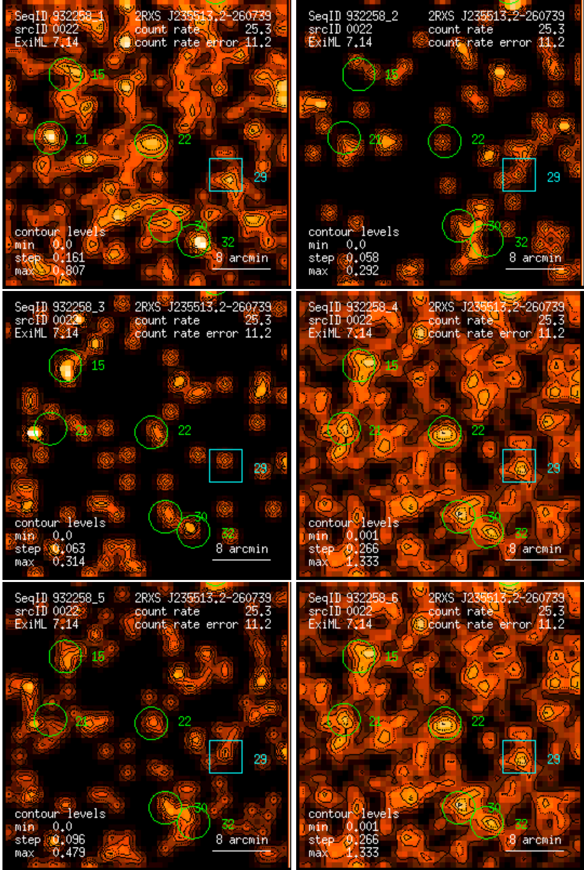
Figure 22: RASS 932258: detection 0022: band rate images, Gaussian filter: (1) PSPC channels 11 – 41, (2) 52 – 90, (3) 91 – 201, (4) 11 – 235, (5) 52 – 201, (6) 11 – 201. Broad band rates in counts/ks. Band rate contour levels in counts/ks/arcmin 2 .
