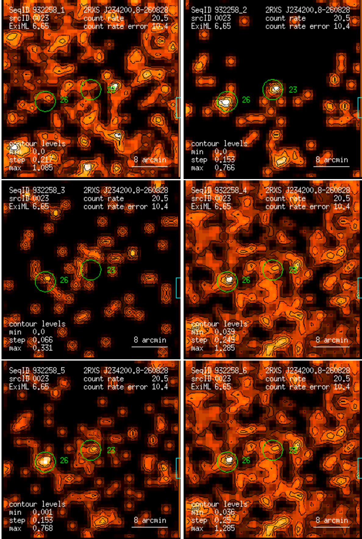
Figure 23: RASS 932258: detection 0023: band rate images, Gaussian filter: (1) PSPC channels 11 – 41, (2) 52 – 90, (3) 91 – 201, (4) 11 – 235, (5) 52 – 201, (6) 11 – 201. Broad band rates in counts/ks. Band rate contour levels in counts/ks/arcmin 2 .
