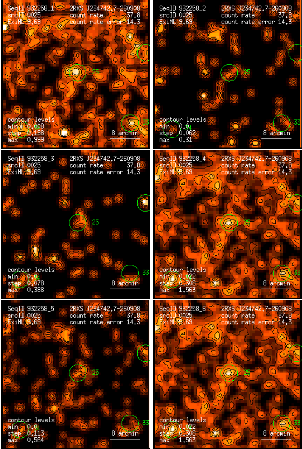
Figure 25: RASS 932258: detection 0025: band rate images, Gaussian filter: (1) PSPC channels 11 – 41, (2) 52 – 90, (3) 91 – 201, (4) 11 – 235, (5) 52 – 201, (6) 11 – 201. Broad band rates in counts/ks. Band rate contour levels in counts/ks/arcmin 2 .
