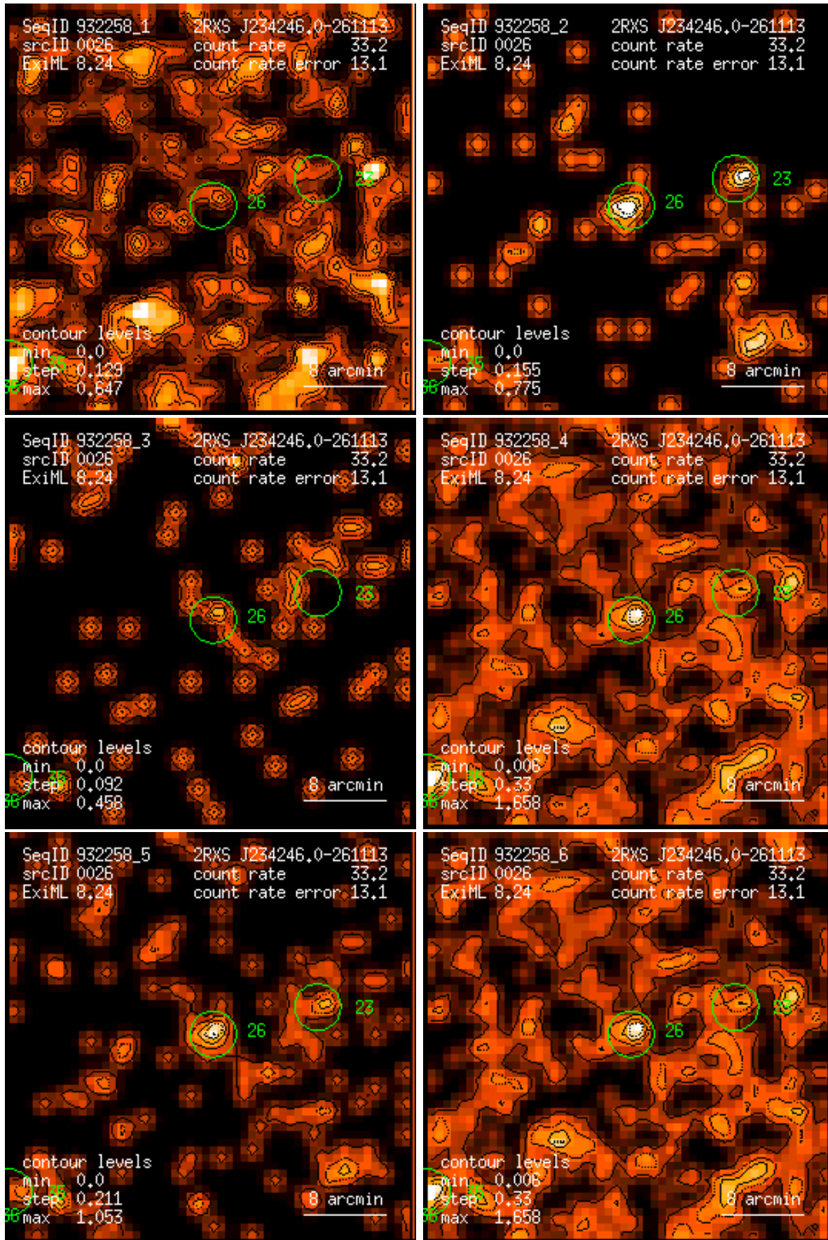
Figure 26: RASS 932258: detection 0026: band rate images, Gaussian filter: (1) PSPC channels 11 – 41, (2) 52 – 90, (3) 91 – 201, (4) 11 – 235, (5) 52 – 201, (6) 11 – 201. Broad band rates in counts/ks. Band rate contour levels in counts/ks/arcmin 2 .
