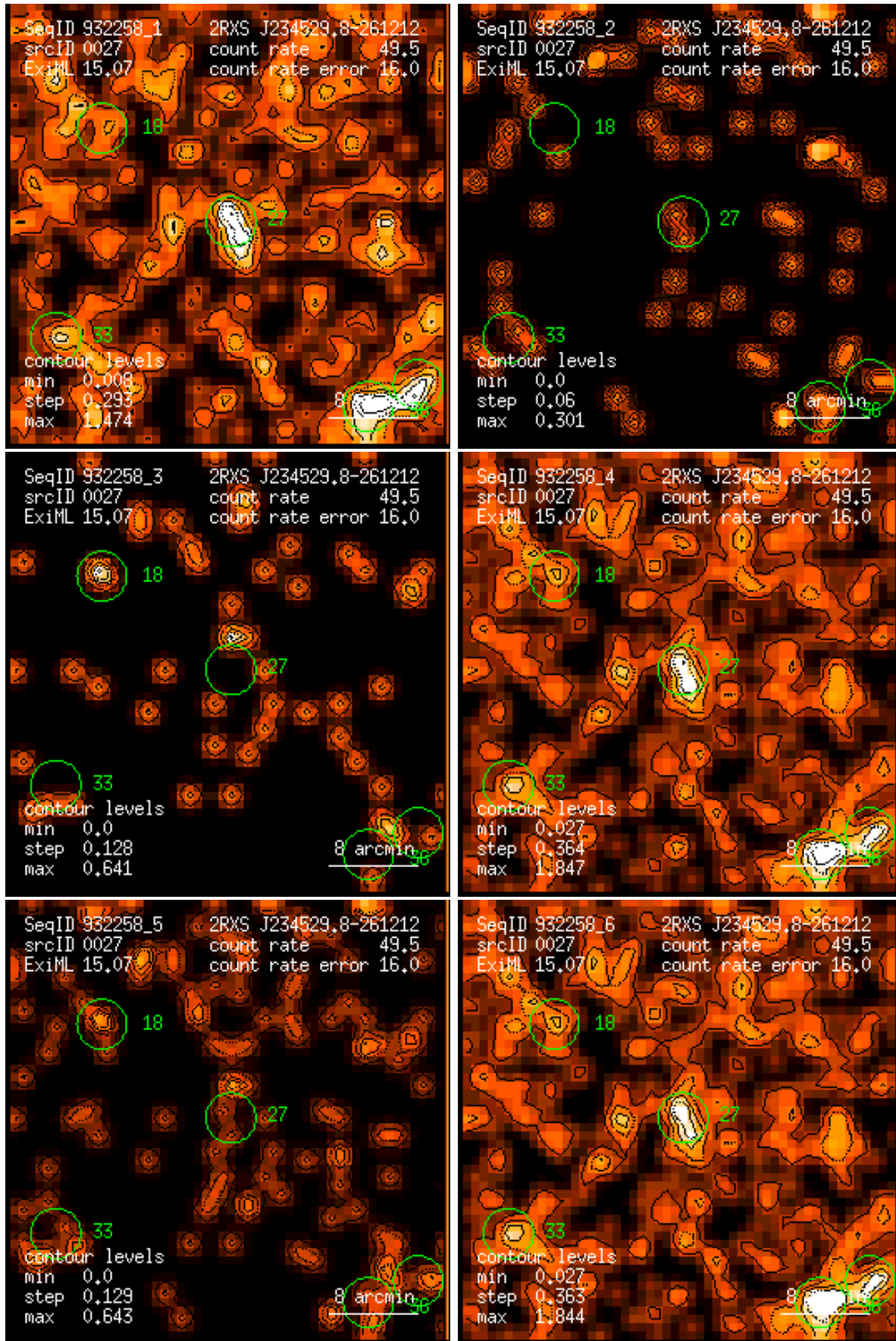
Figure 27: RASS 932258: detection 0027: band rate images, Gaussian filter: (1) PSPC channels 11 – 41, (2) 52 – 90, (3) 91 – 201, (4) 11 – 235, (5) 52 – 201, (6) 11 – 201. Broad band rates in counts/ks. Band rate contour levels in counts/ks/arcmin 2 .
