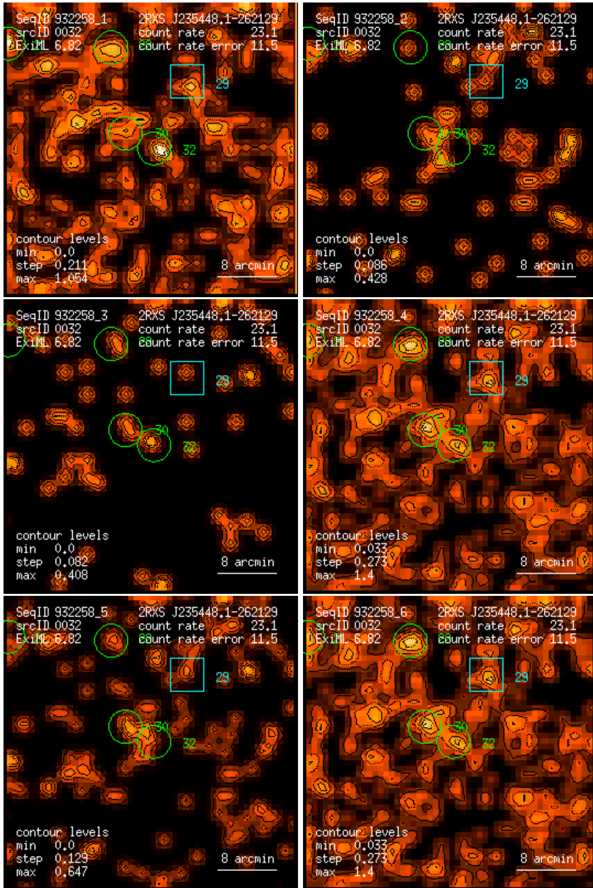
Figure 32: RASS 932258: detection 0032: band rate images, Gaussian filter: (1) PSPC channels 11 – 41, (2) 52 – 90, (3) 91 – 201, (4) 11 – 235, (5) 52 – 201, (6) 11 – 201. Broad band rates in counts/ks. Band rate contour levels in counts/ks/arcmin 2 .
