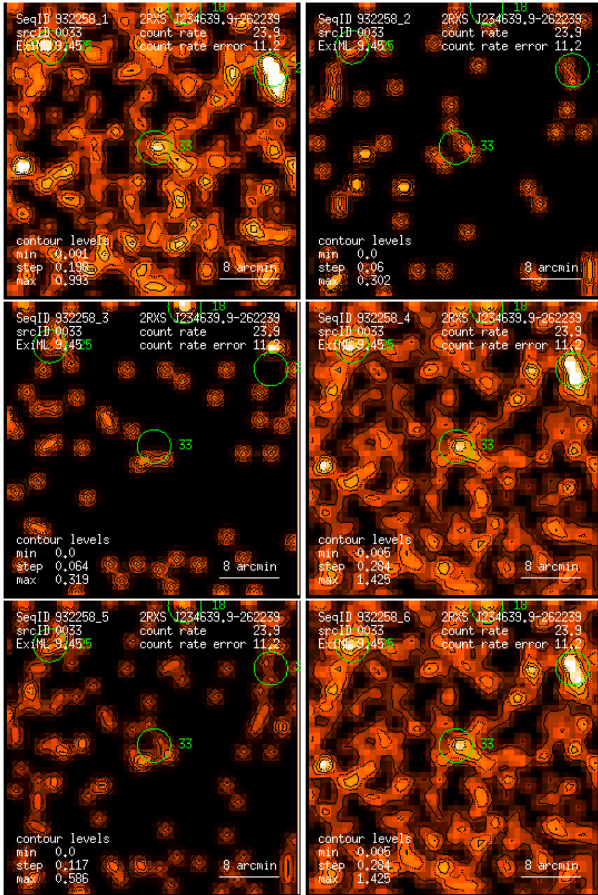
Figure 33: RASS 932258: detection 0033: band rate images, Gaussian filter: (1) PSPC channels 11 – 41, (2) 52 – 90, (3) 91 – 201, (4) 11 – 235, (5) 52 – 201, (6) 11 – 201. Broad band rates in counts/ks. Band rate contour levels in counts/ks/arcmin 2 .
