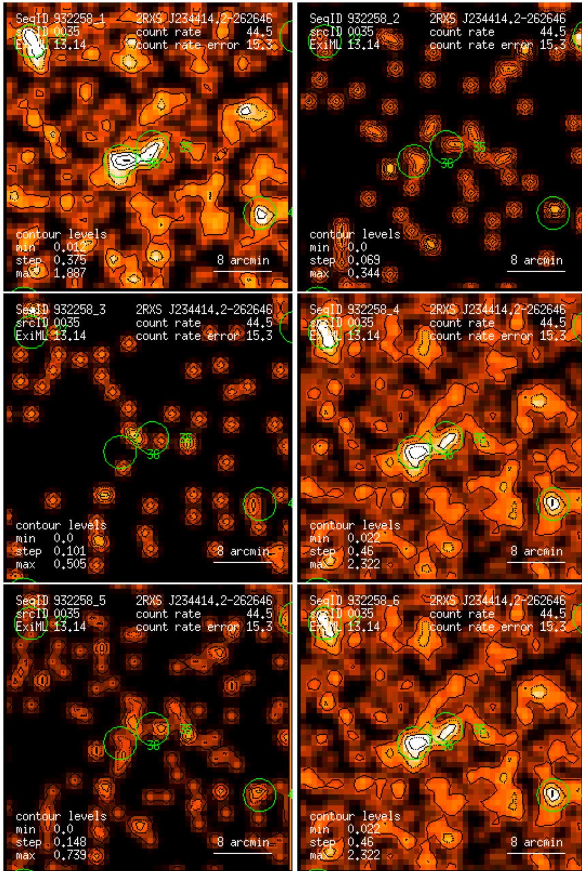
Figure 35: RASS 932258: detection 0035: band rate images, Gaussian filter: (1) PSPC channels 11 – 41, (2) 52 – 90, (3) 91 – 201, (4) 11 – 235, (5) 52 – 201, (6) 11 – 201. Broad band rates in counts/ks. Band rate contour levels in counts/ks/arcmin 2 .
