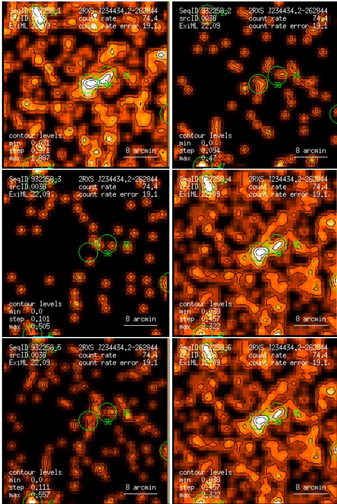
Figure 36: RASS 932258: detection 0036: band rate images, Gaussian filter: (1) PSPC channels 11 – 41, (2) 52 – 90, (3) 91 – 201, (4) 11 – 235, (5) 52 – 201, (6) 11 – 201. Broad band rates in counts/ks. Band rate contour levels in counts/ks/arcmin 2 .
