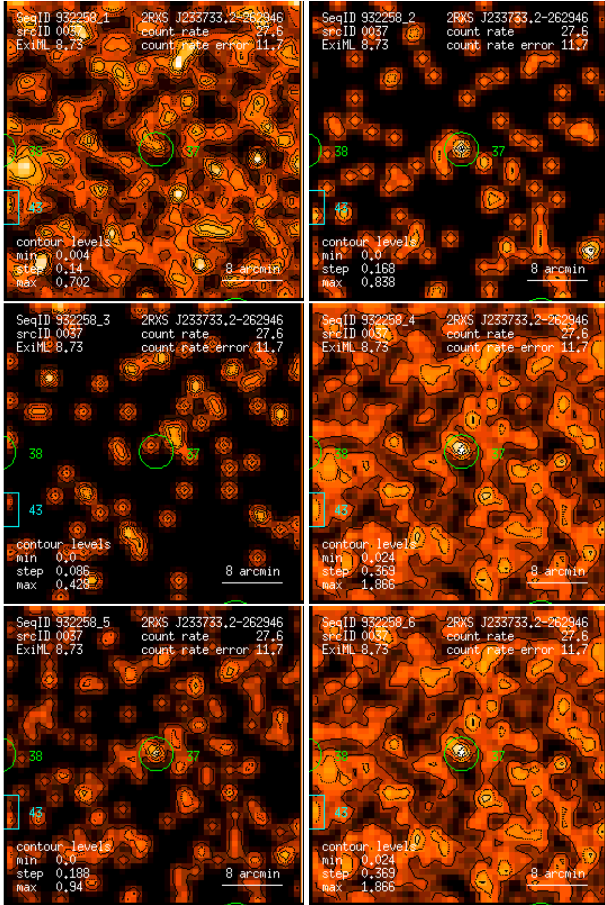
Figure 37: RASS 932258: detection 0037: band rate images, Gaussian filter: (1) PSPC channels 11 – 41, (2) 52 – 90, (3) 91 – 201, (4) 11 – 235, (5) 52 – 201, (6) 11 – 201. Broad band rates in counts/ks. Band rate contour levels in counts/ks/arcmin 2 .
