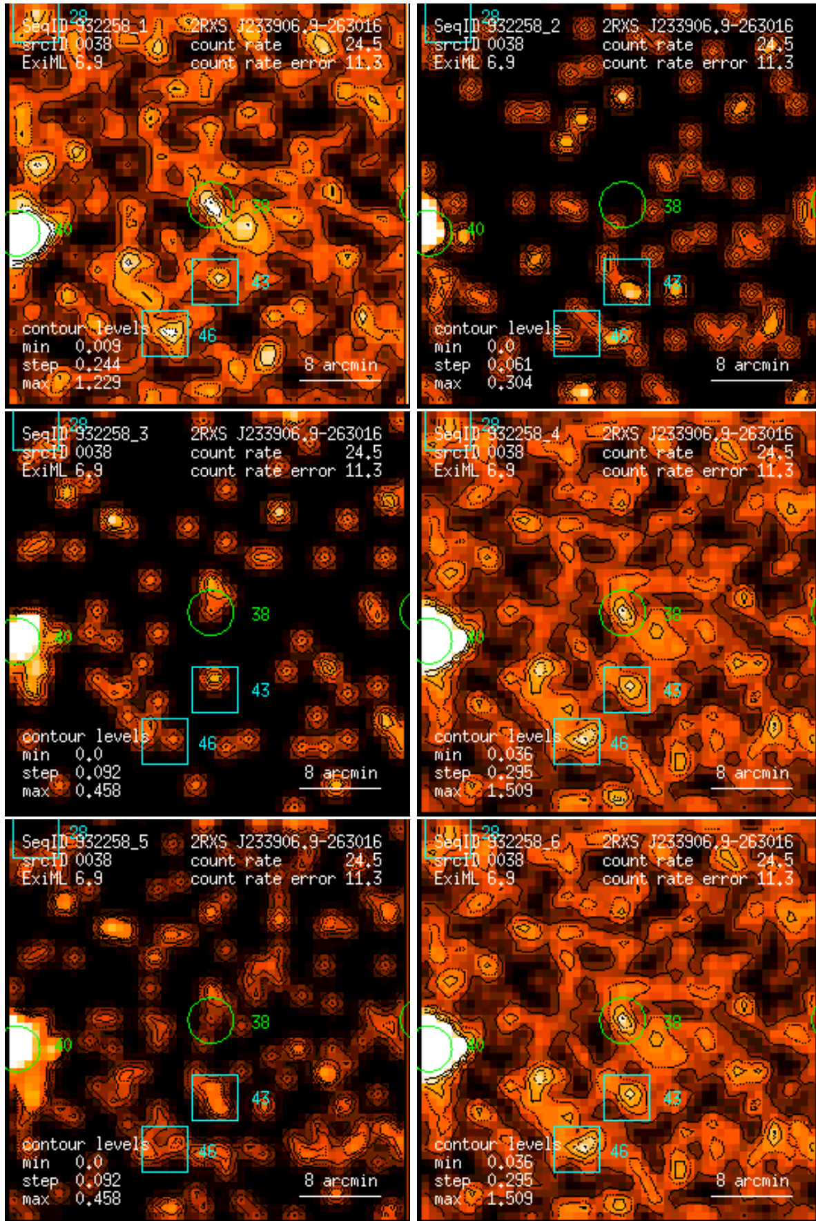
Figure 38: RASS 932258: detection 0038: band rate images, Gaussian filter: (1) PSPC channels 11 – 41, (2) 52 – 90, (3) 91 – 201, (4) 11 – 235, (5) 52 – 201, (6) 11 – 201. Broad band rates in counts/ks. Band rate contour levels in counts/ks/arcmin 2 .
