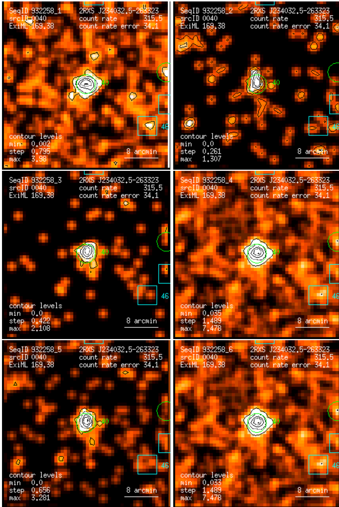
Figure 40: RASS 932258: detection 0040: band rate images, Gaussian filter: (1) PSPC channels 11 – 41, (2) 52 – 90, (3) 91 – 201, (4) 11 – 235, (5) 52 – 201, (6) 11 – 201. Broad band rates in counts/ks. Band rate contour levels in counts/ks/arcmin 2 .
