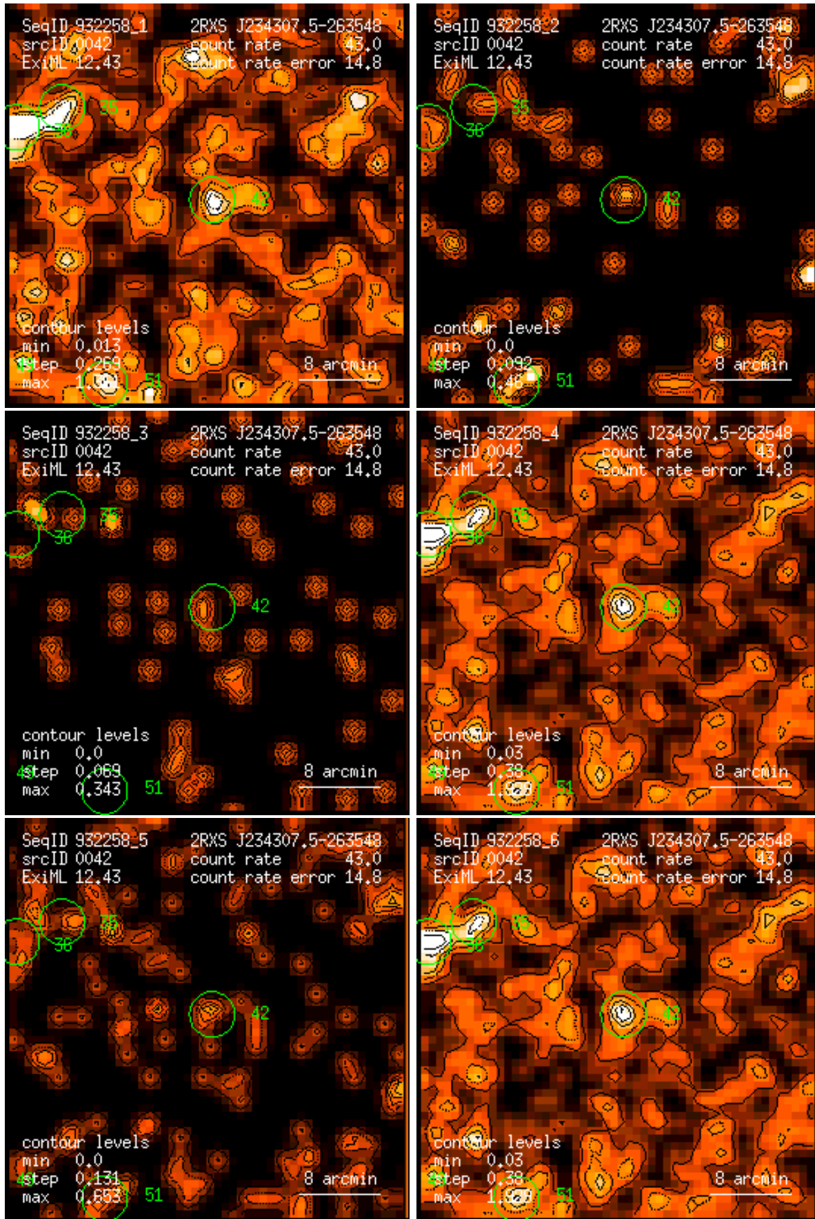
Figure 42: RASS 932258: detection 0042: band rate images, Gaussian filter: (1) PSPC channels 11 – 41, (2) 52 – 90, (3) 91 – 201, (4) 11 – 235, (5) 52 – 201, (6) 11 – 201. Broad band rates in counts/ks. Band rate contour levels in counts/ks/arcmin 2 .
