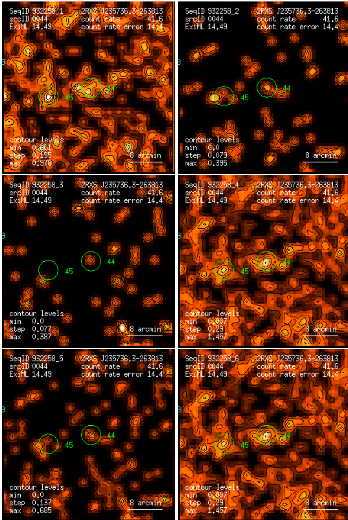
Figure 44: RASS 932258: detection 0044: band rate images, Gaussian filter: (1) PSPC channels 11 – 41, (2) 52 – 90, (3) 91 – 201, (4) 11 – 235, (5) 52 – 201, (6) 11 – 201. Broad band rates in counts/ks. Band rate contour levels in counts/ks/arcmin 2 .
