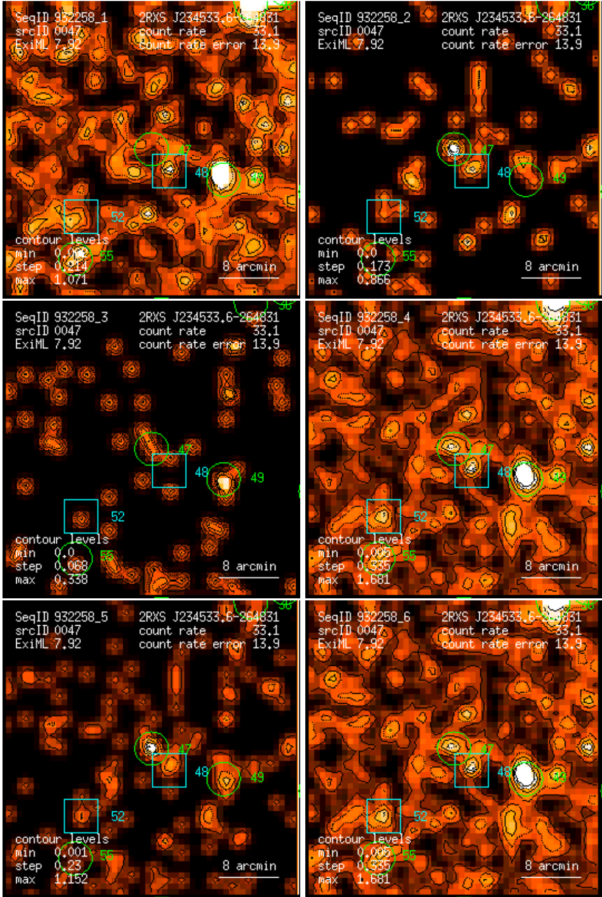
Figure 47: RASS 932258: detection 0047: band rate images, Gaussian filter: (1) PSPC channels 11 – 41, (2) 52 – 90, (3) 91 – 201, (4) 11 – 235, (5) 52 – 201, (6) 11 – 201. Broad band rates in counts/ks. Band rate contour levels in counts/ks/arcmin 2 .
