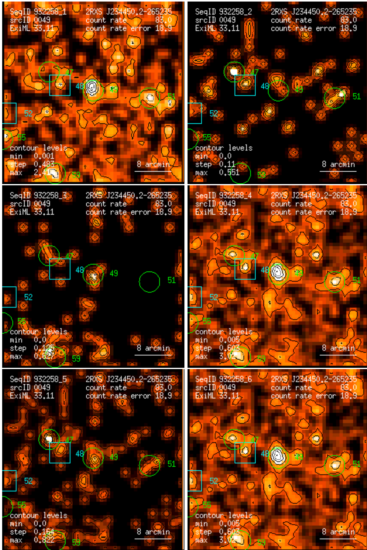
Figure 49: RASS 932258: detection 0049: band rate images, Gaussian filter: (1) PSPC channels 11 – 41, (2) 52 – 90, (3) 91 – 201, (4) 11 – 235, (5) 52 – 201, (6) 11 – 201. Broad band rates in counts/ks. Band rate contour levels in counts/ks/arcmin 2 .
