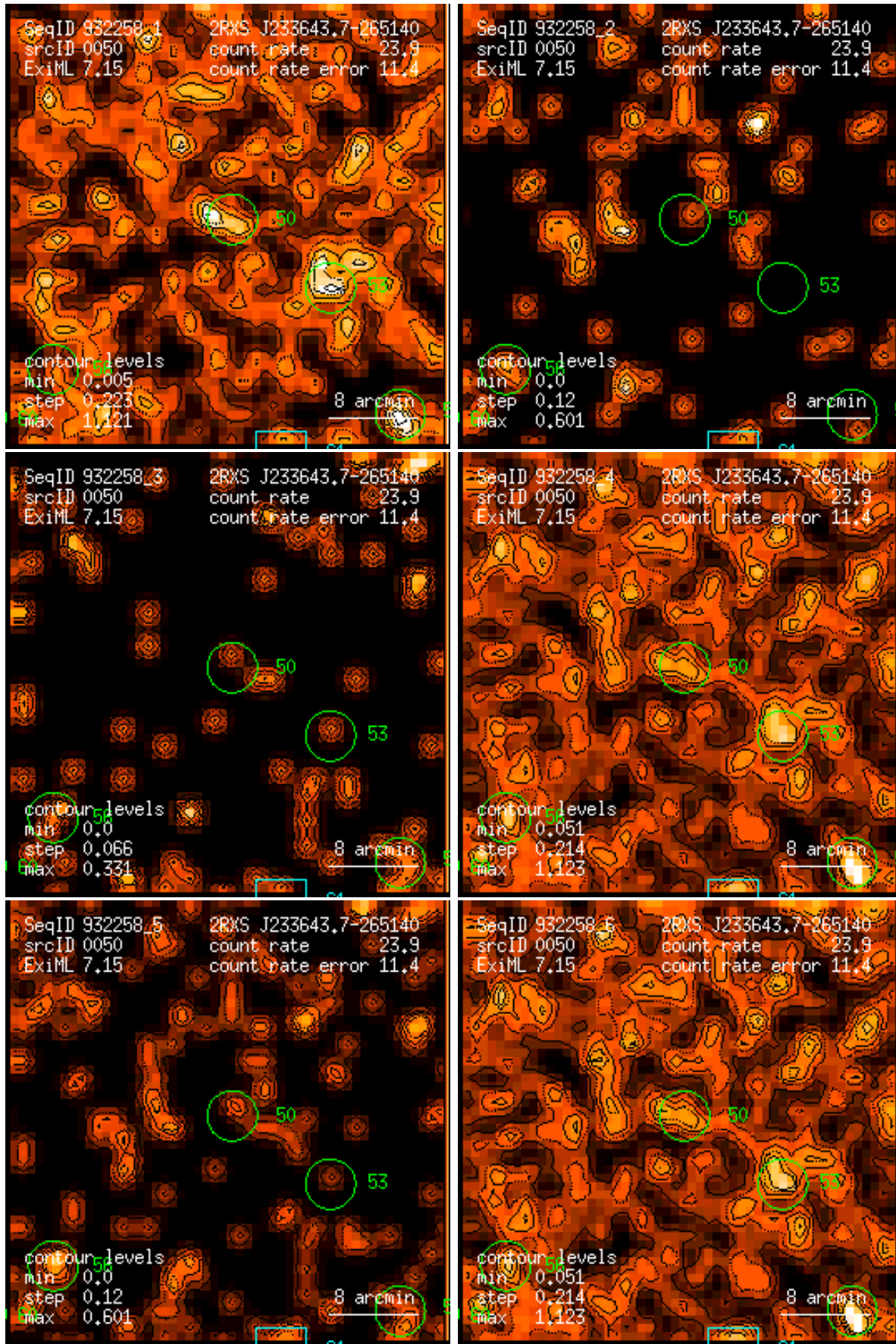
Figure 50: RASS 932258: detection 0050: band rate images, Gaussian filter: (1) PSPC channels 11 – 41, (2) 52 – 90, (3) 91 – 201, (4) 11 – 235, (5) 52 – 201, (6) 11 – 201. Broad band rates in counts/ks. Band rate contour levels in counts/ks/arcmin 2 .
