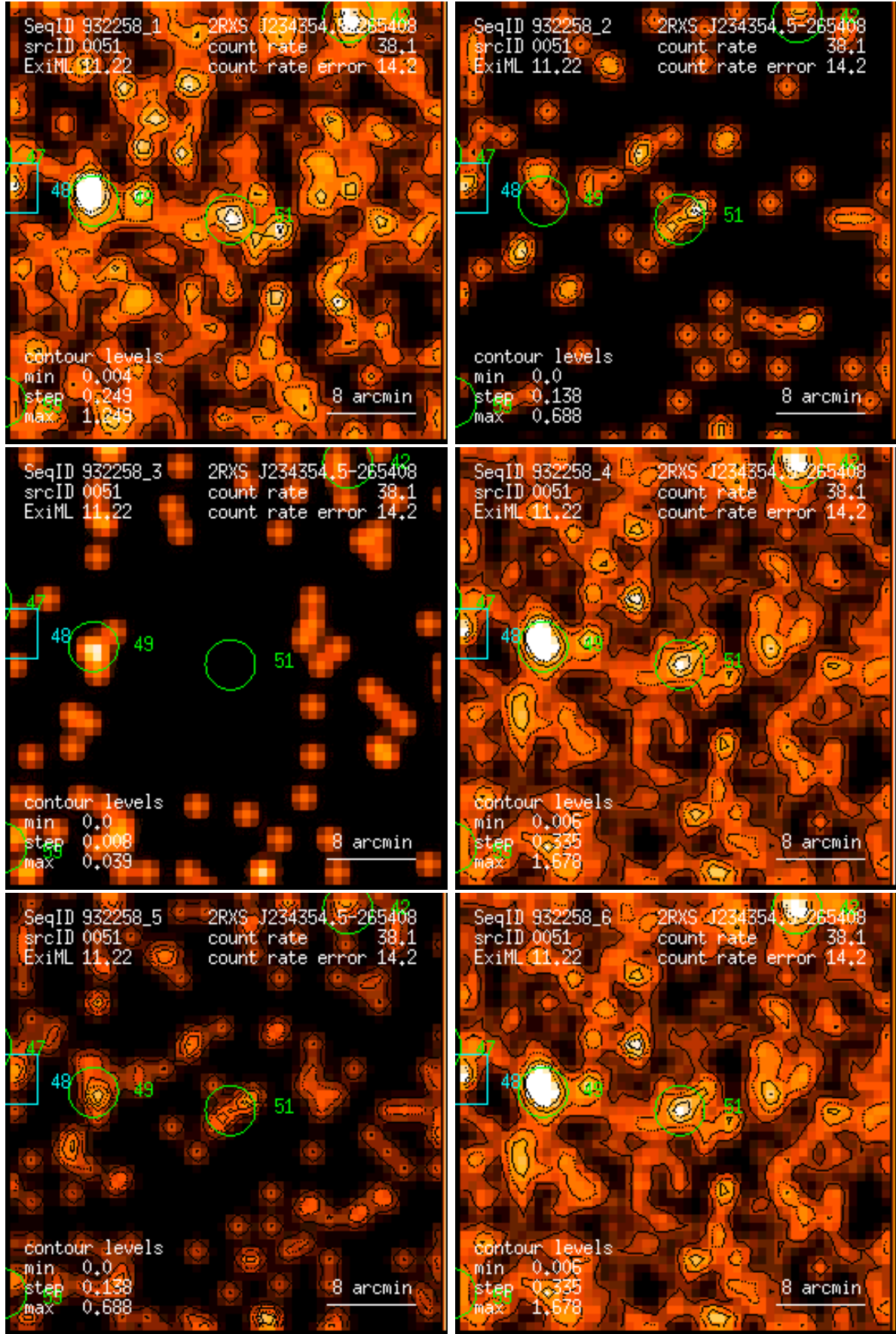
Figure 51: RASS 932258: detection 0051: band rate images, Gaussian filter: (1) PSPC channels 11 – 41, (2) 52 – 90, (3) 91 – 201, (4) 11 – 235, (5) 52 – 201, (6) 11 – 201. Broad band rates in counts/ks. Band rate contour levels in counts/ks/arcmin 2 .
