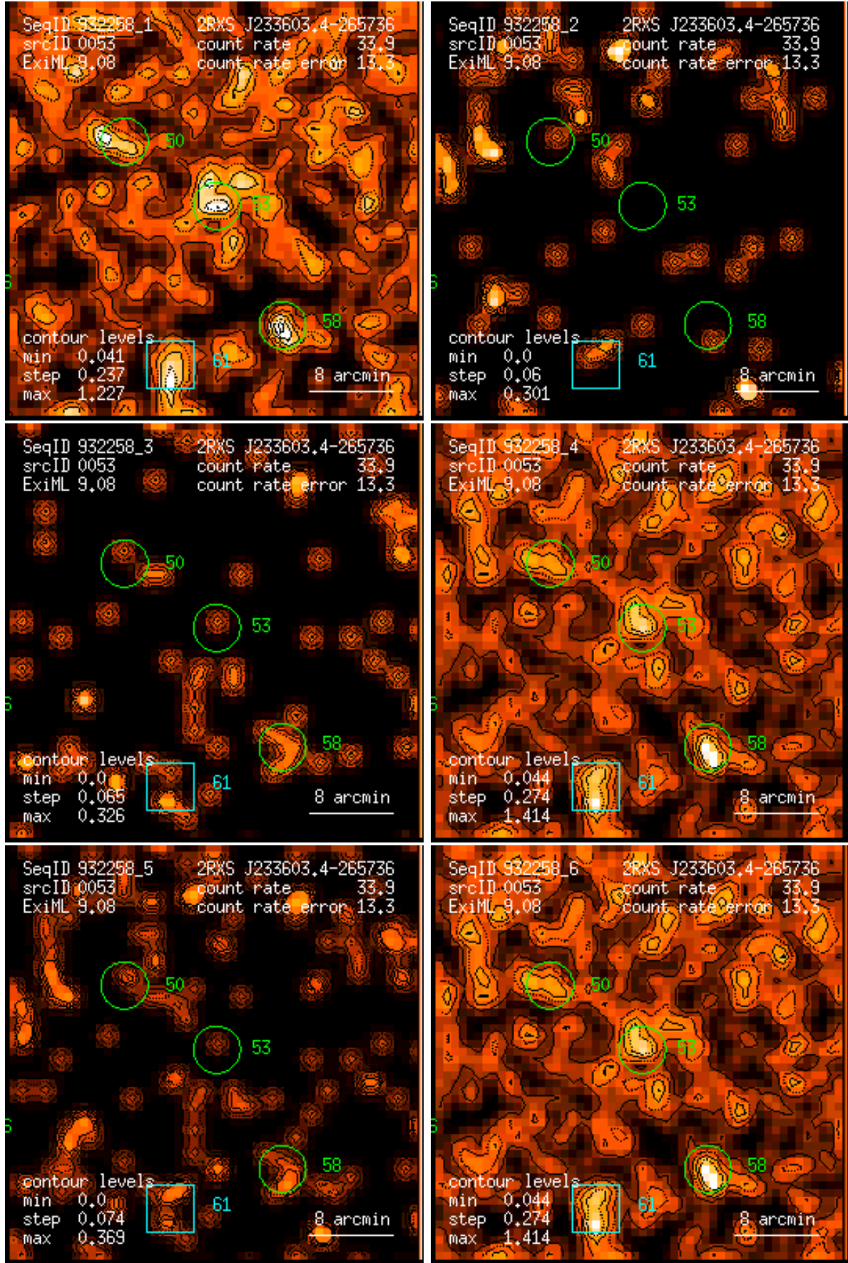
Figure 53: RASS 932258: detection 0053: band rate images, Gaussian filter: (1) PSPC channels 11 – 41, (2) 52 – 90, (3) 91 – 201, (4) 11 – 235, (5) 52 – 201, (6) 11 – 201. Broad band rates in counts/ks. Band rate contour levels in counts/ks/arcmin 2 .
