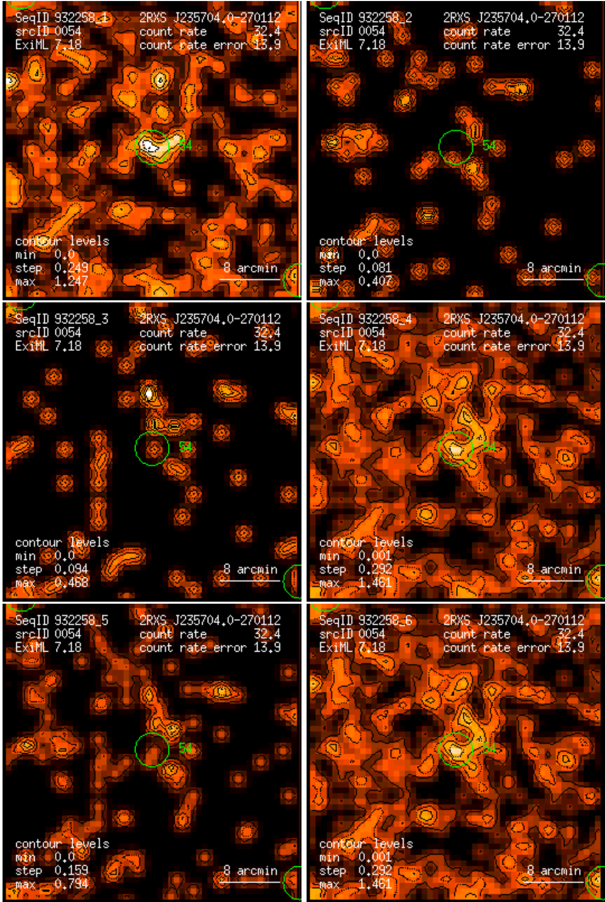
Figure 54: RASS 932258: detection 0054: band rate images, Gaussian filter: (1) PSPC channels 11 – 41, (2) 52 – 90, (3) 91 – 201, (4) 11 – 235, (5) 52 – 201, (6) 11 – 201. Broad band rates in counts/ks. Band rate contour levels in counts/ks/arcmin 2 .
