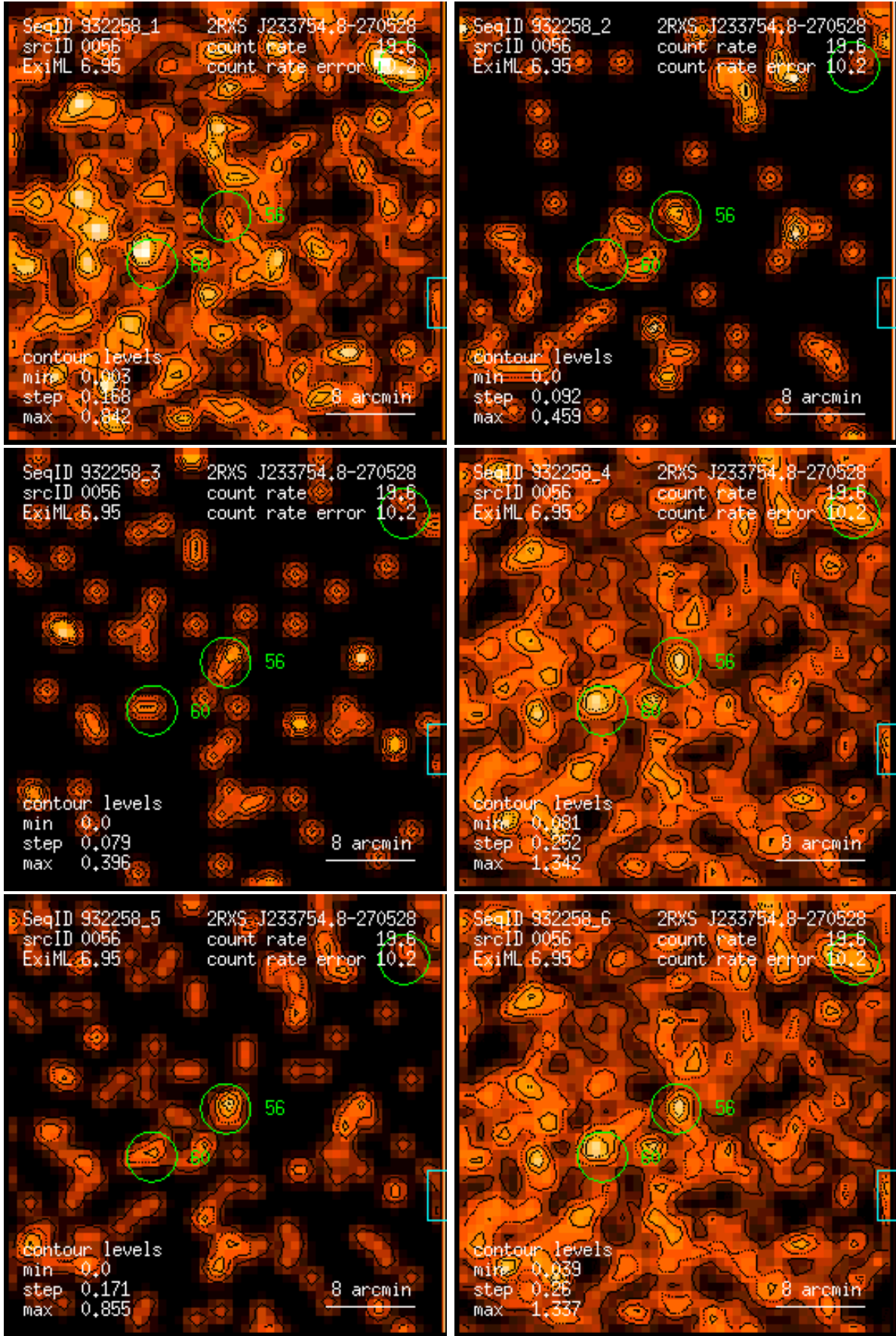
Figure 56: RASS 932258: detection 0056: band rate images, Gaussian filter: (1) PSPC channels 11 – 41, (2) 52 – 90, (3) 91 – 201, (4) 11 – 235, (5) 52 – 201, (6) 11 – 201. Broad band rates in counts/ks. Band rate contour levels in counts/ks/arcmin 2 .
